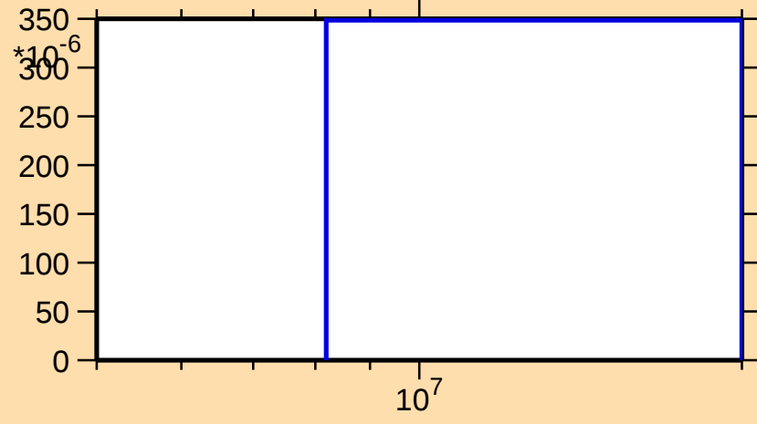
\sigma vs. E for ^{127}\text{Te}(n,d)
