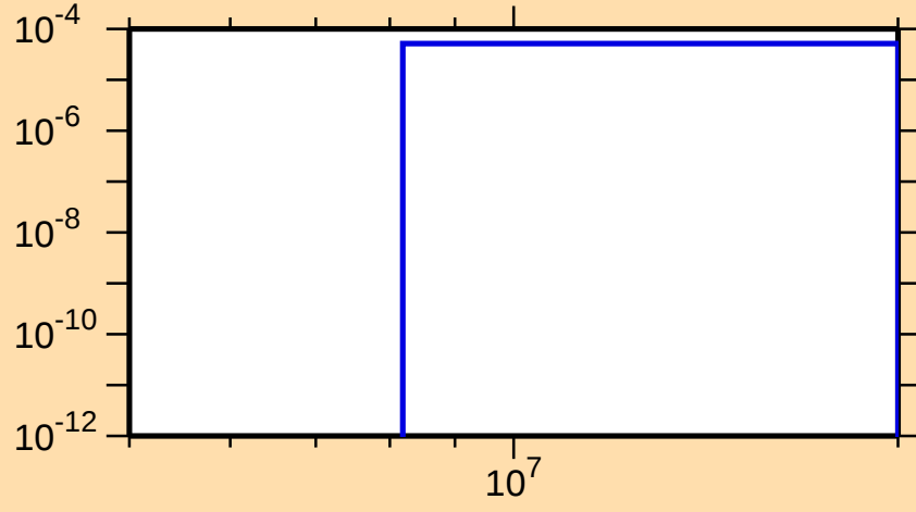
\sigma vs. E for ^{127}\text{Te}(n,n\alpha)
