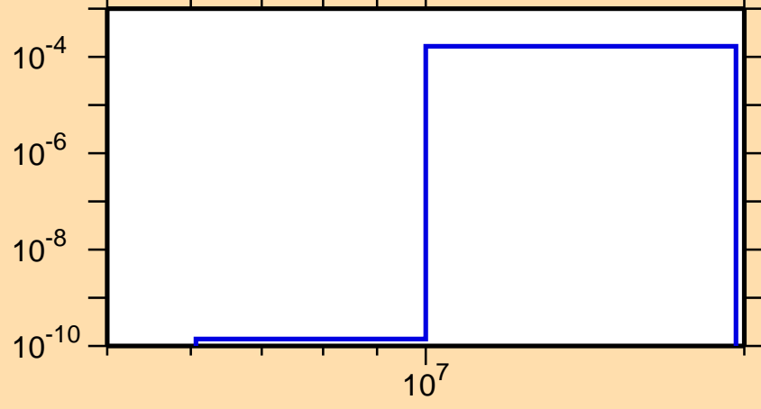
\sigma vs. E for ^{128}\text{Te}(n,n\alpha)
