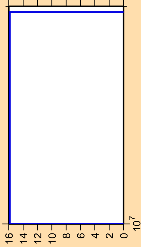
\Delta\sigma/\sigma vs. E for ^{128}\text{Te}(n,nd)
