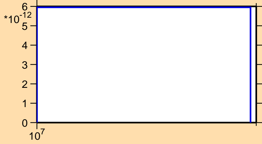
\sigma vs. E for ^{128}\text{Te}(n,nd)
