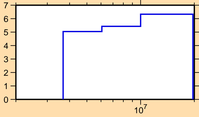
\Delta\sigma/\sigma vs. E for ^{128}\text{Te}(n,el.)
