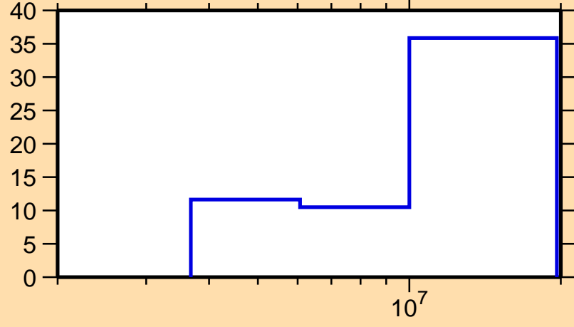
\Delta\sigma/\sigma vs. E for ^{128}\text{Te}(n,ncont.)
