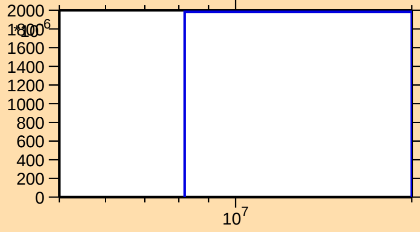
\sigma vs. E for ^{128}\text{Te}(n,3n)
