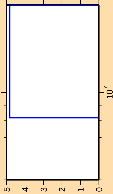
\Delta\sigma/\sigma vs. E for ^{128}\text{Te}(n,nt)
