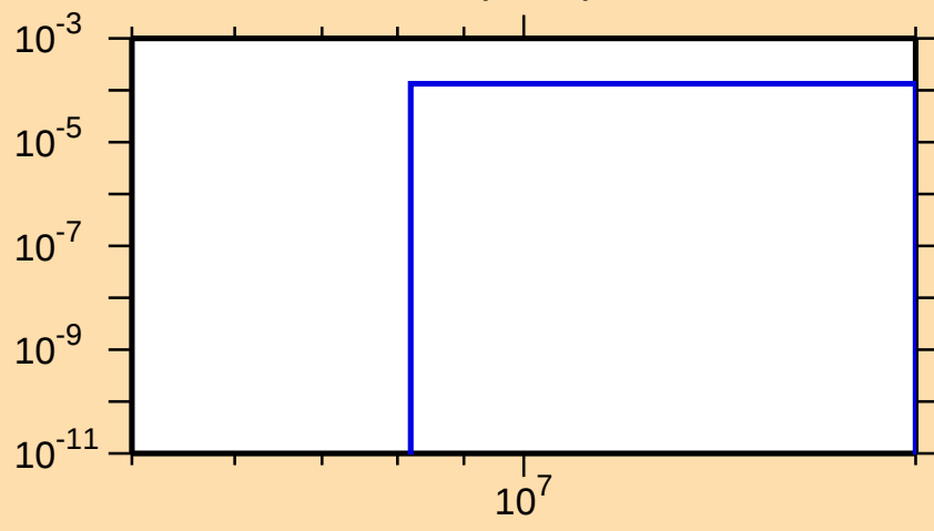
\sigma vs. E for ^{128}\text{Te}(n,n\alpha)
