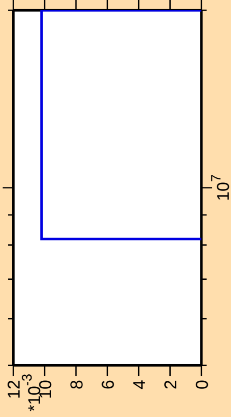
\Delta\sigma/\sigma vs. E for ^{128}\text{Te}(n,2np)
