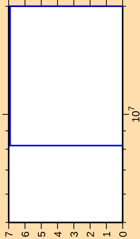
\Delta\sigma/\sigma vs. E for ^{128}\text{Te}(n,2n\alpha)
