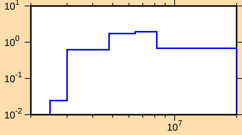
\sigma vs. E for ^{128}\text{Te}(n,n\text{cont.})
