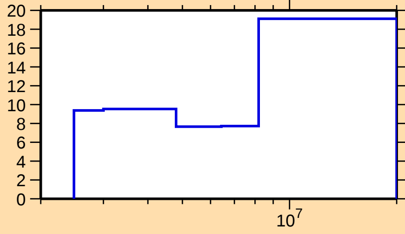
\Delta\sigma/\sigma vs. E for ^{128}\text{Te}(\text{n},\text{inel.})
