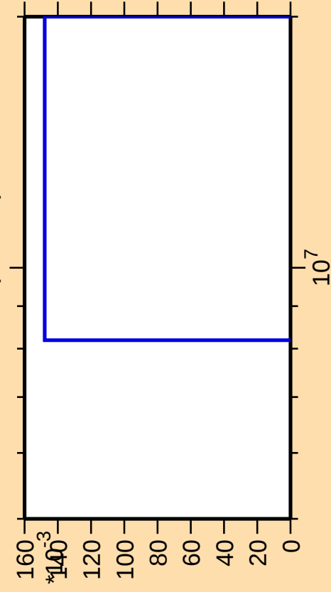
\Delta\sigma/\sigma vs. E for ^{128}\text{Te}(n,\text{He3})
