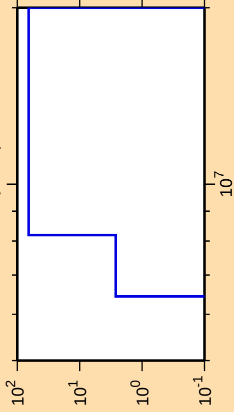
\Delta\sigma/\sigma vs. E for ^{128}\text{Te}(n,n\alpha)
