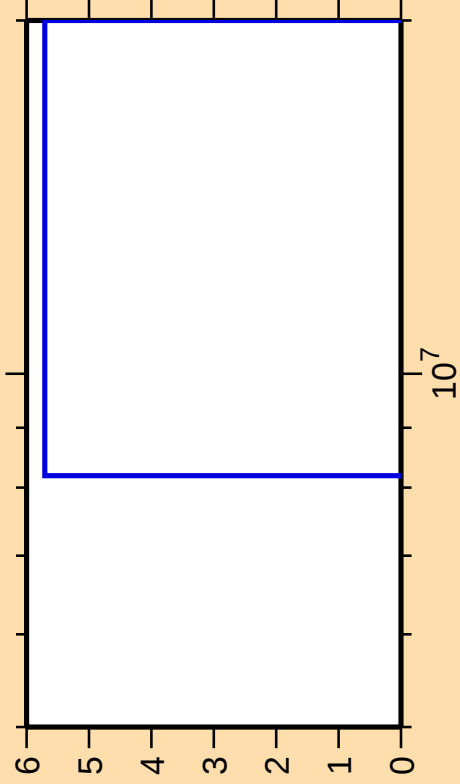
\Delta\sigma/\sigma vs. E for ^{128}\text{Te}(n,2n)
