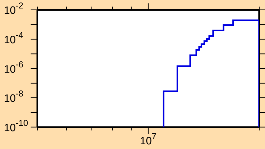
\sigma vs. E for ^{129}\text{Te}(n,d)
