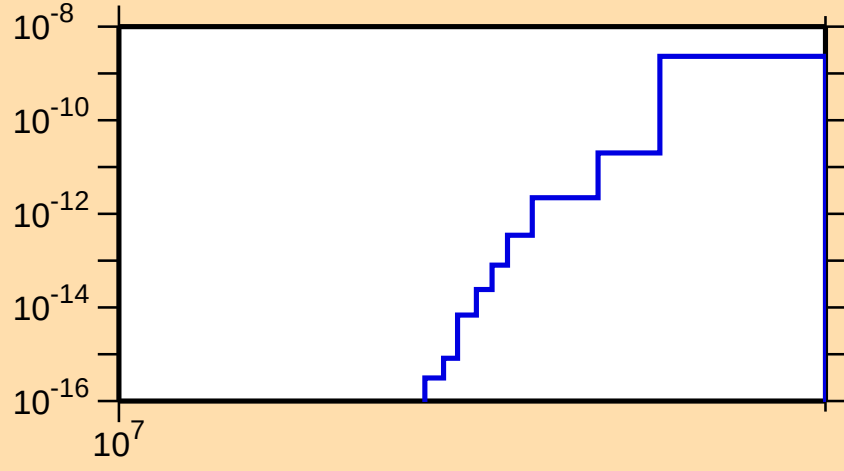
\sigma vs. E for ^{129}\text{Te}(n,2n\alpha)
