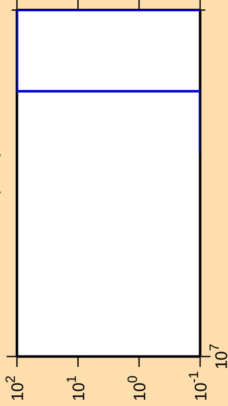
\Delta\sigma/\sigma vs. E for ^{129}\text{Te}(n,\text{nt})
