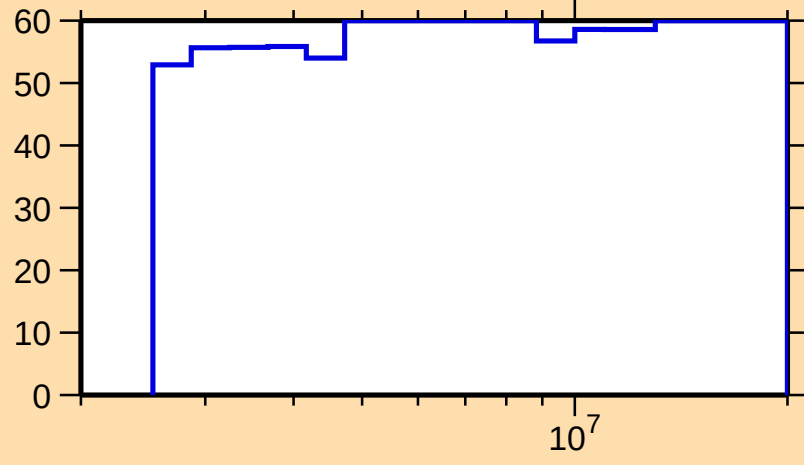
\Delta\sigma/\sigma vs. E for ^{129}\text{Te}(n,\gamma)
