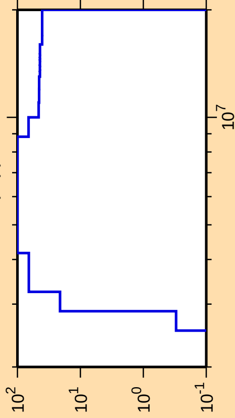
\Delta\sigma/\sigma vs. E for ^{129}\text{Te}(n,p)
