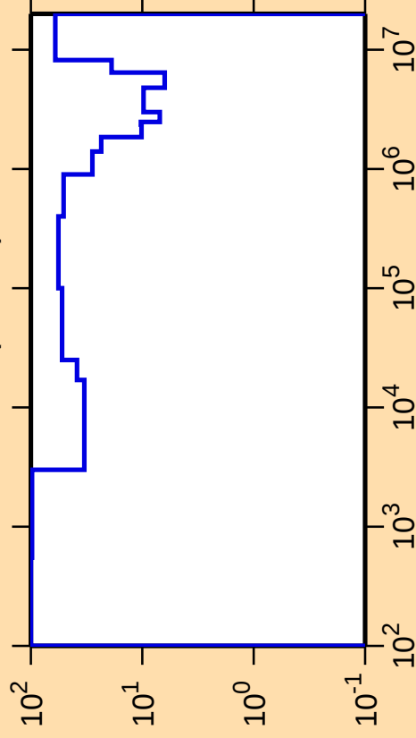
\Delta\sigma/\sigma vs. E for ^{129}\text{Te}(n,\text{inel.})
