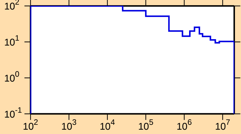
\Delta\sigma/\sigma vs. E for ^{129}\text{Te}(n,\text{el.})
