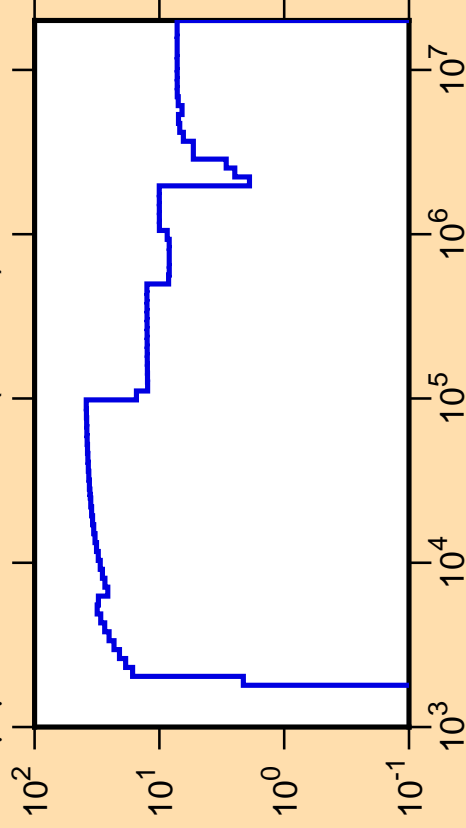
\Delta\mu/\mu vs. E for ^{130}\text{Te}(\text{mt251})
