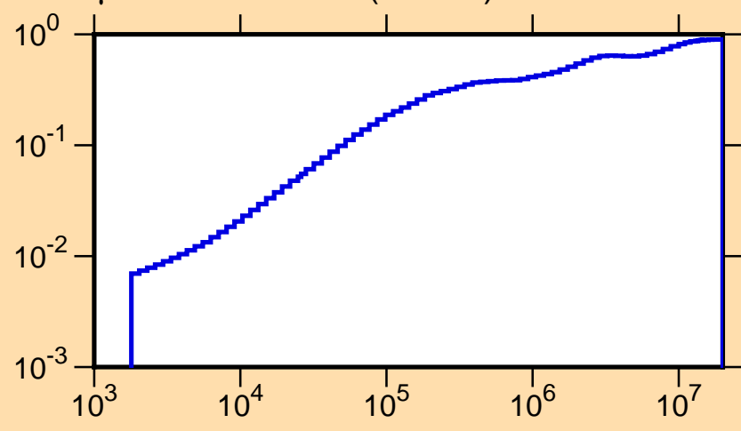
\mu vs. E for ^{130}\text{Te}(\text{mt251})
