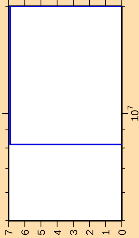
\Delta\sigma/\sigma vs. E for ^{130}\text{Te}(n,nt)
