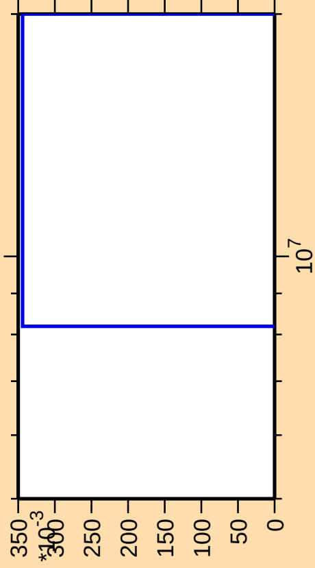
\Delta\sigma/\sigma vs. E for ^{130}\text{Te}(n,2n\alpha)
