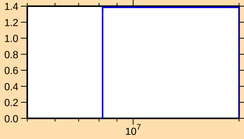
\sigma vs. E for ^{130}\text{Te}(n,2n)
