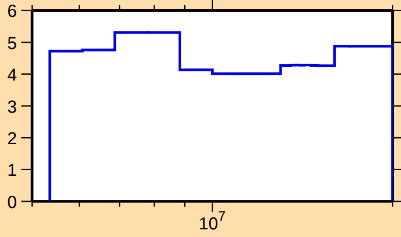
\Delta\sigma/\sigma vs. E for ^{131}\text{Te}(n,\text{nonel.})
