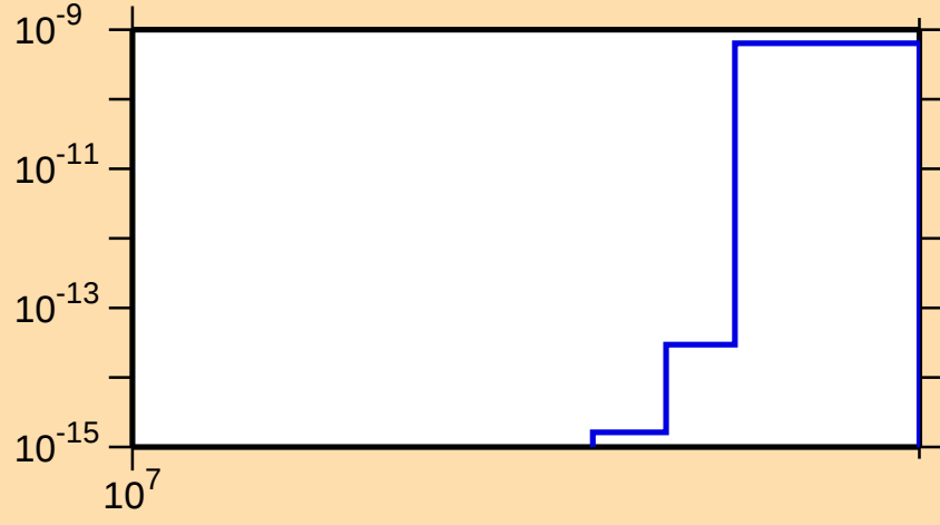
\sigma vs. E for ^{131}\text{Te}(n,\text{nt})
