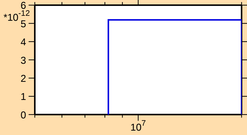
\sigma vs. E for ^{131}\text{Te}(n,nt)
