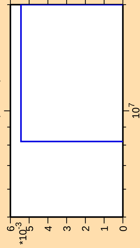
\Delta\sigma/\sigma vs. E for ^{131}\text{Te}(n,\text{He}3)
