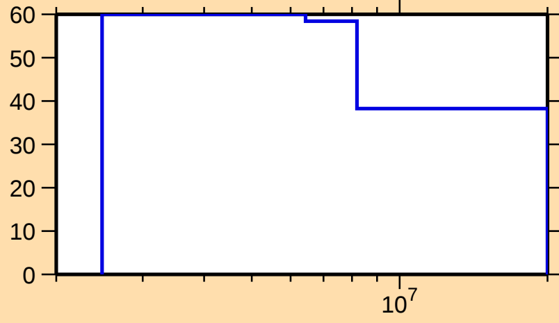
\Delta\sigma/\sigma vs. E for ^{131}\text{Te}(n,n_1)
