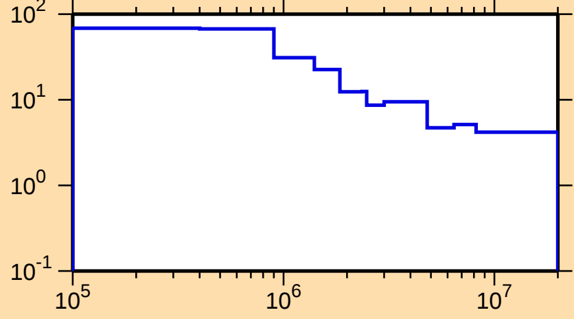
\Delta\sigma/\sigma vs. E for ^{131}\text{Te}(n,\text{nonel.})
