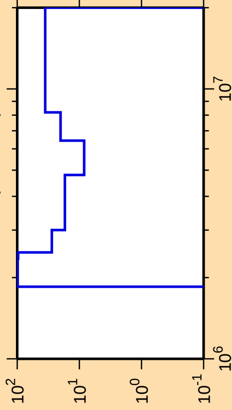
\Delta\sigma/\sigma vs. E for ^{131}\text{Te}(n,\text{ncont.})
