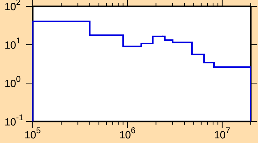
\Delta\sigma/\sigma vs. E for ^{131}\text{Te}(n,\text{tot.})
