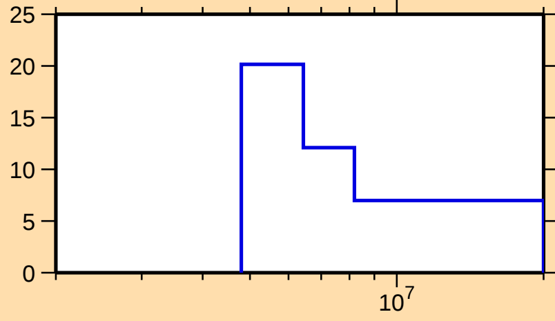
\Delta\sigma/\sigma vs. E for ^{131}\text{Te}(n,2n)
