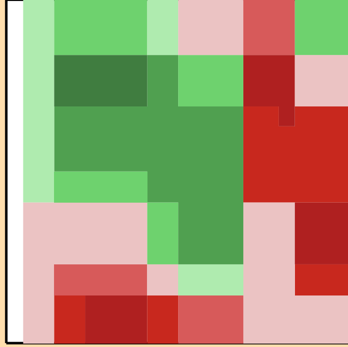
\Delta\sigma/\sigma vs. E for ^{131}\text{Te}(n,2n)
