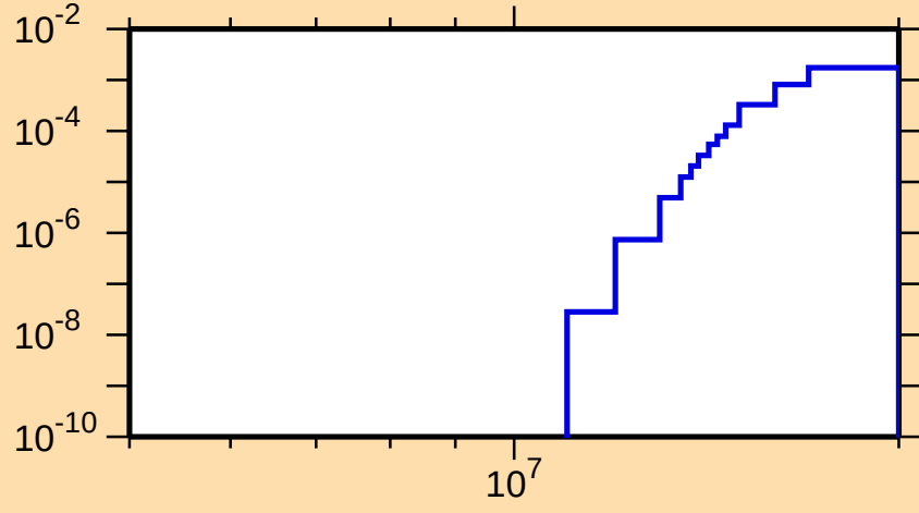
\sigma vs. E for ^{131}\text{Te}(n,d)
