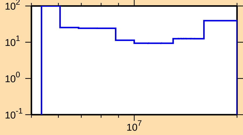
\Delta\sigma/\sigma vs. E for ^{131}\text{Te}(n,2n)
