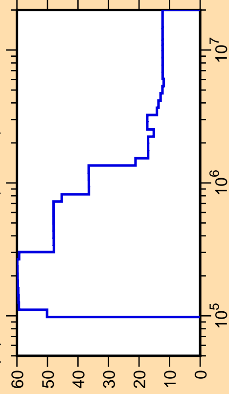
\Delta\mu/\mu vs. E for ^{132}\text{Te}(\text{mt251})
