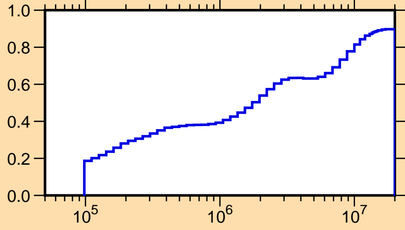
\mu vs. E for ^{132}\text{Te}(\text{mt251})
