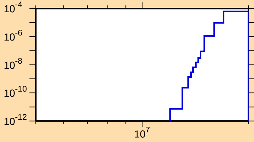
\sigma vs. E for ^{132}\text{Te}(n,t)
