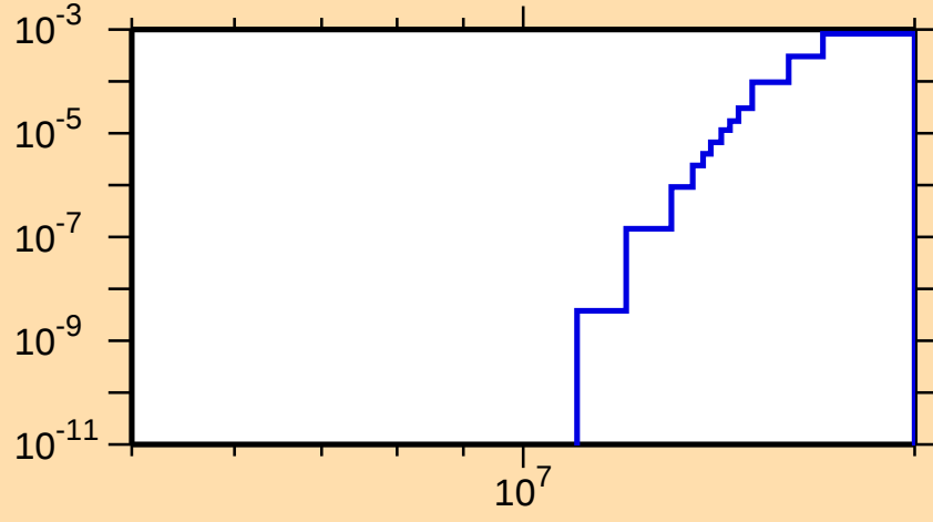
\sigma vs. E for ^{132}\text{Te}(n,d)
