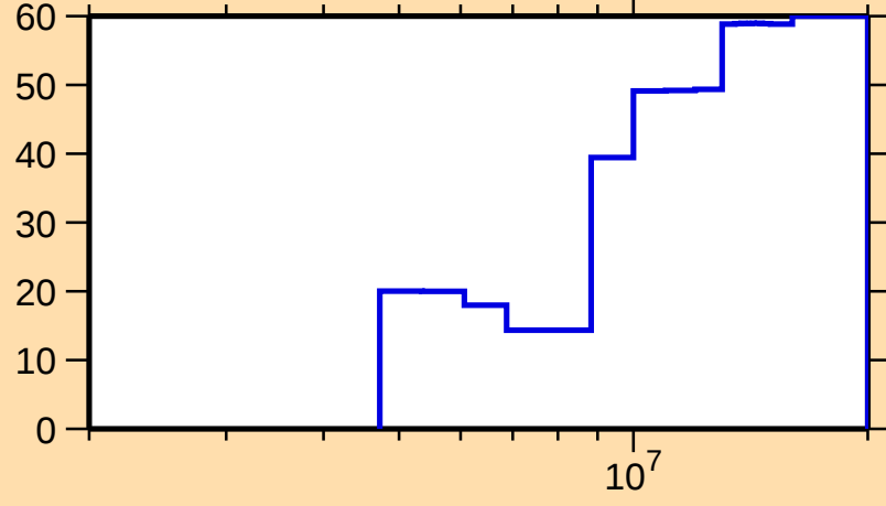
\Delta\sigma/\sigma vs. E for ^{132}\text{Te}(n,n\text{cont.})
