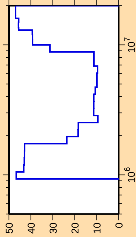
\Delta\sigma/\sigma vs. E for ^{132}\text{Te}(n,\text{inel.})
