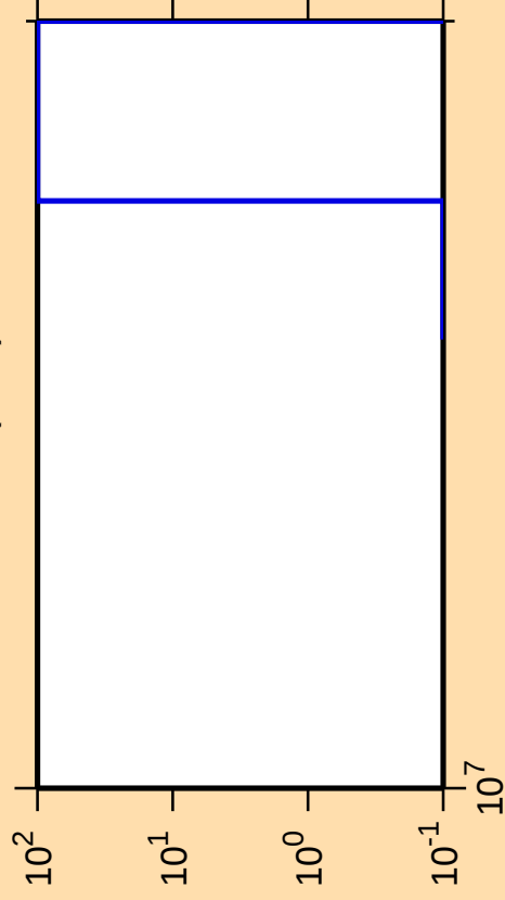
\Delta\sigma/\sigma vs. E for ^{132}\text{Te}(n,\text{nt})
