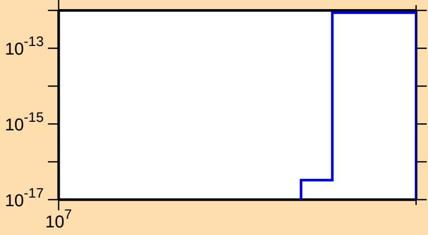
\sigma vs. E for ^{132}\text{Te}(n,2n\alpha)
