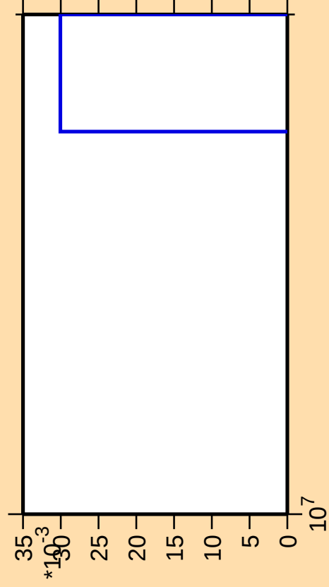
\Delta\sigma/\sigma vs. E for ^{132}\text{Te}(n,2np)
