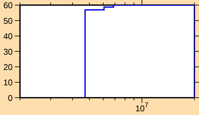
\Delta\sigma/\sigma vs. E for ^{132}\text{Te}(n,n_1)
