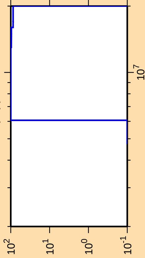
\Delta\sigma/\sigma vs. E for ^{132}\text{Te}(n,p)
