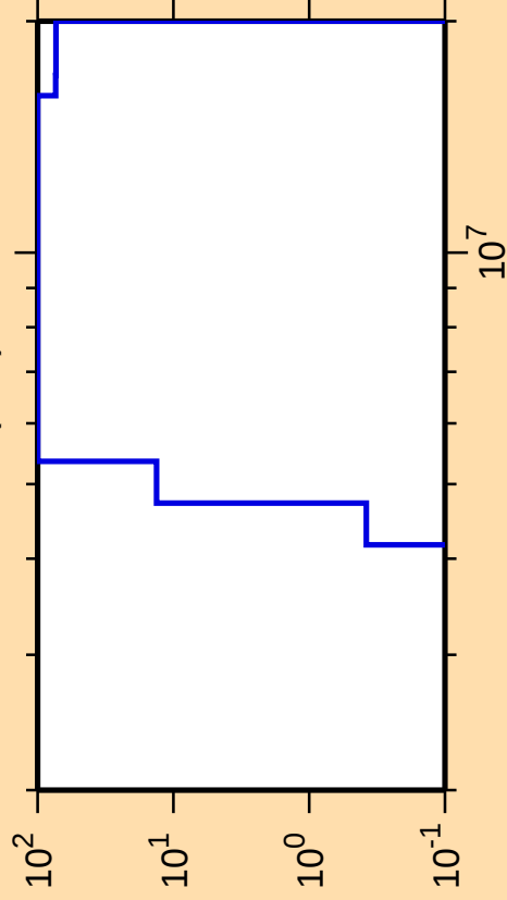
\Delta\sigma/\sigma vs. E for ^{132}\text{Te}(n,\alpha)
