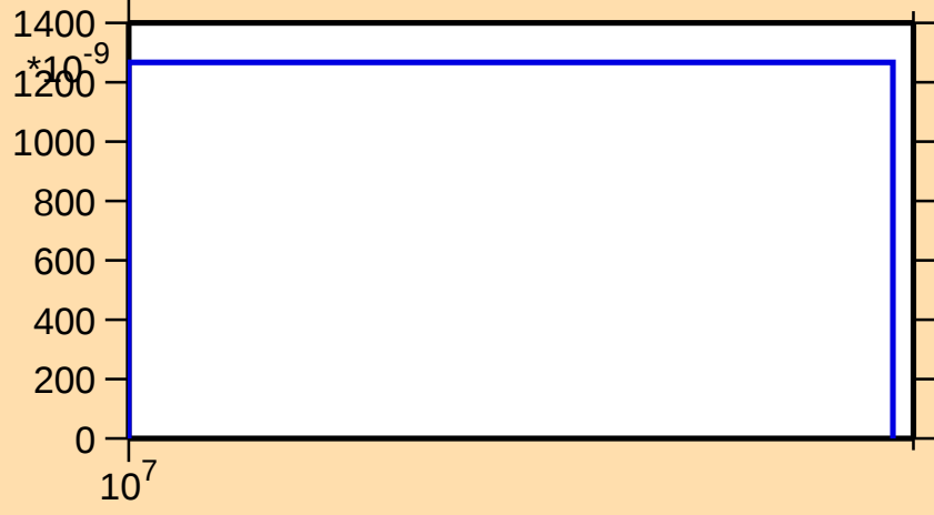
\sigma vs. E for ^{132}\text{Te}(n,t)
