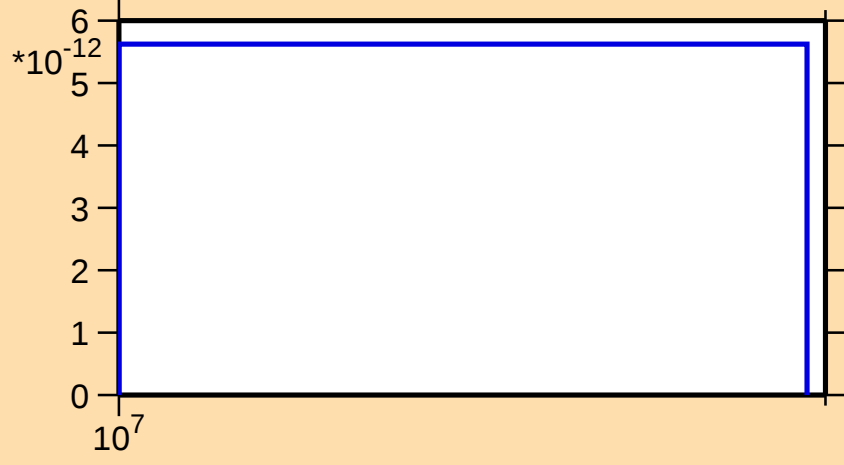
\sigma vs. E for ^{132}\text{Te}(n,\text{nt})
