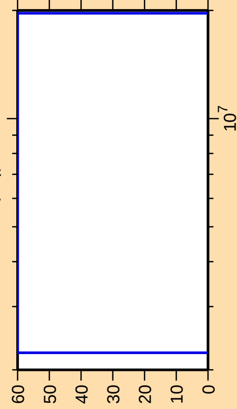
\Delta\sigma/\sigma vs. E for ^{132}\text{Te}(n,\gamma)
