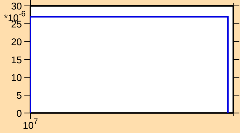
\sigma vs. E for ^{132}\text{Te}(n,np)
