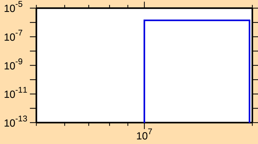
\sigma vs. E for ^{132}\text{Te}(n,n\alpha)
