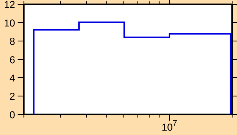
\Delta\sigma/\sigma vs. E for ^{132}\text{Te}(n,n\text{onel.})
