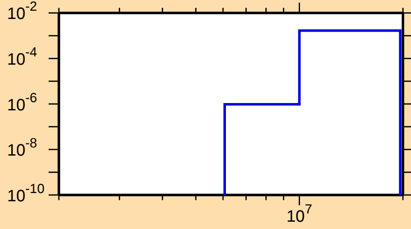
\sigma vs. E for ^{132}\text{Te}(n,p)
