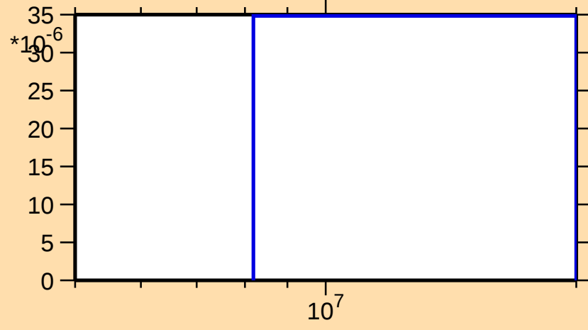
\sigma vs. E for ^{132}\text{Te}(n,d)
