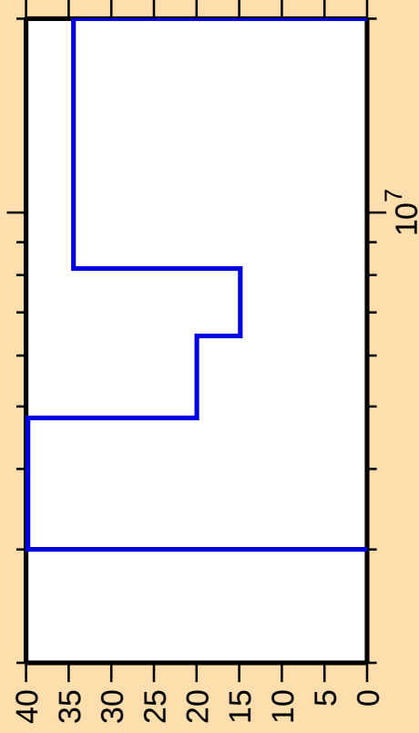
\Delta\sigma/\sigma vs. E for ^{132}\text{Te}(n,\text{ncont.})
