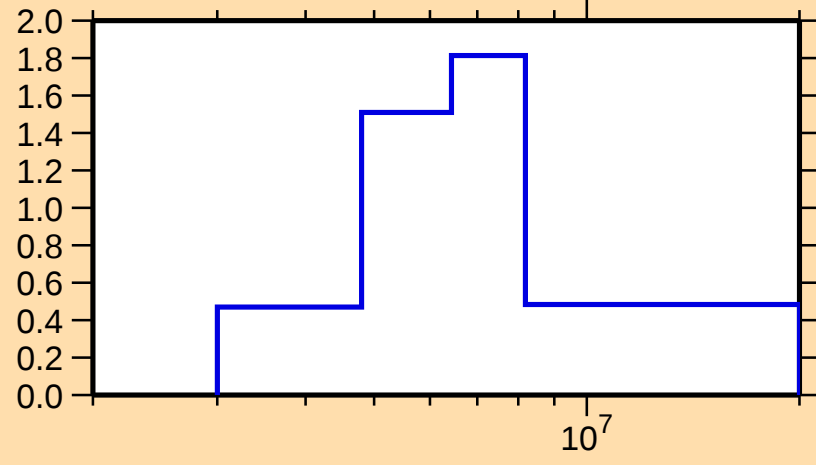
\sigma vs. E for ^{132}\text{Te}(n,n\text{cont.})
