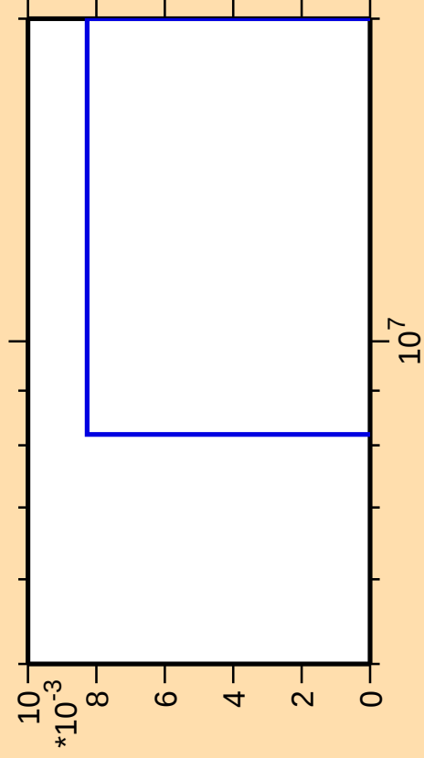
\Delta\sigma/\sigma vs. E for ^{132}\text{Te}(n,2n\alpha)
