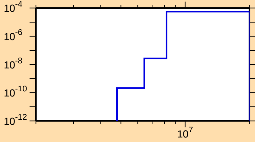
\sigma vs. E for ^{132}\text{Te}(n,\alpha)
