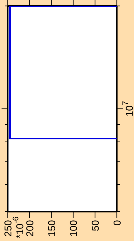
\Delta\sigma/\sigma vs. E for ^{132}\text{Te}(n,2np)
