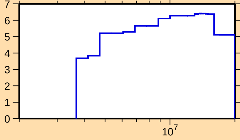
\Delta\sigma/\sigma vs. E for ^{133}\text{Te}(n,n\text{onel.})
