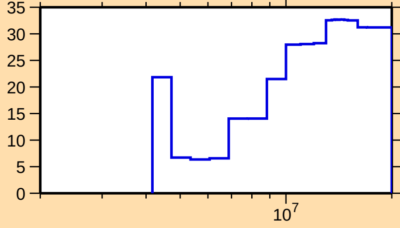
\Delta\sigma/\sigma vs. E for ^{133}\text{Te}(n,n\text{cont.})
