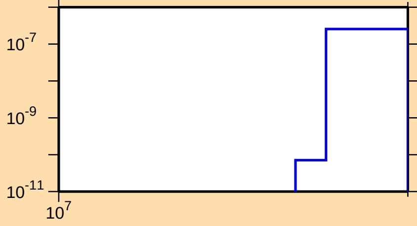
\sigma vs. E for ^{133}\text{Te}(n,\text{nd})
