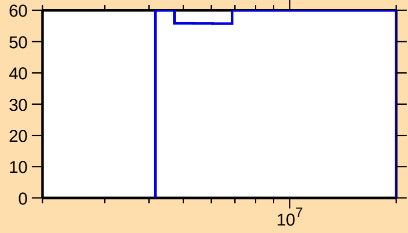
\Delta\sigma/\sigma vs. E for ^{133}\text{Te}(n,\gamma)
