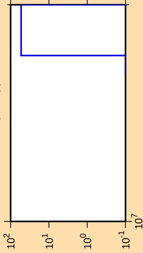
\Delta\sigma/\sigma vs. E for ^{133}\text{Te}(n,2np)
