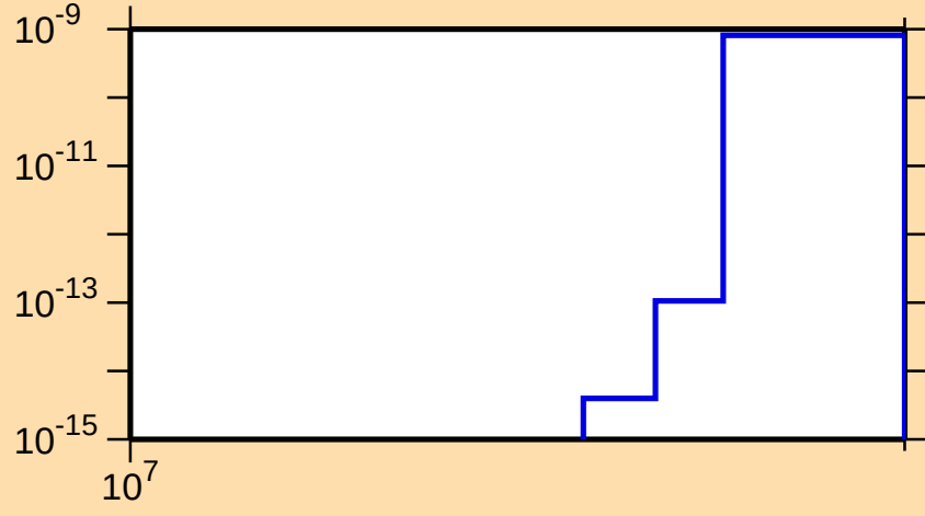
\sigma vs. E for ^{133}\text{Te}(n,\text{nt})
