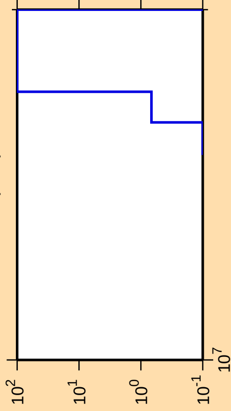
\Delta\sigma/\sigma vs. E for ^{133}\text{Te}(n,\text{nt})
