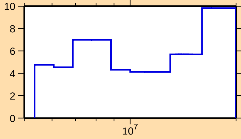
\Delta\sigma/\sigma vs. E for ^{133}\text{Te}(n,\text{el.})
