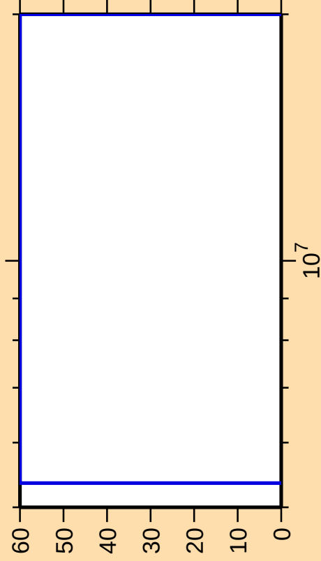
\Delta\sigma/\sigma vs. E for ^{133}\text{Te}(n,\alpha)
