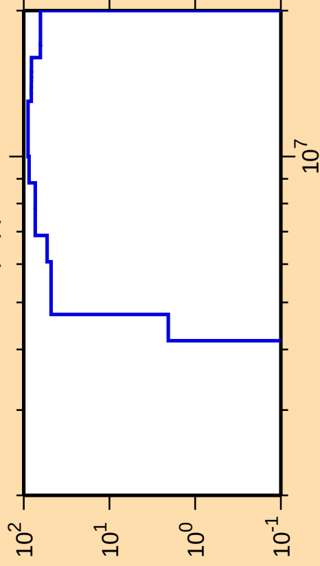
\Delta\sigma/\sigma vs. E for ^{133}\text{Te}(n,p)
