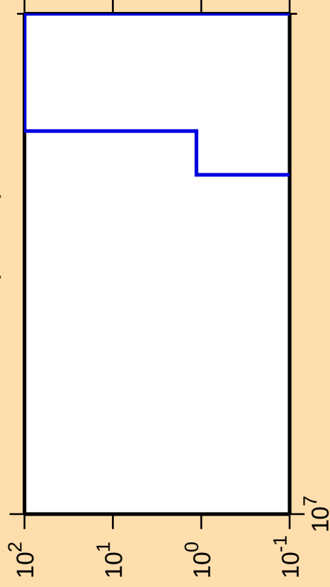
\Delta\sigma/\sigma vs. E for ^{133}\text{Te}(n,2n\alpha)
