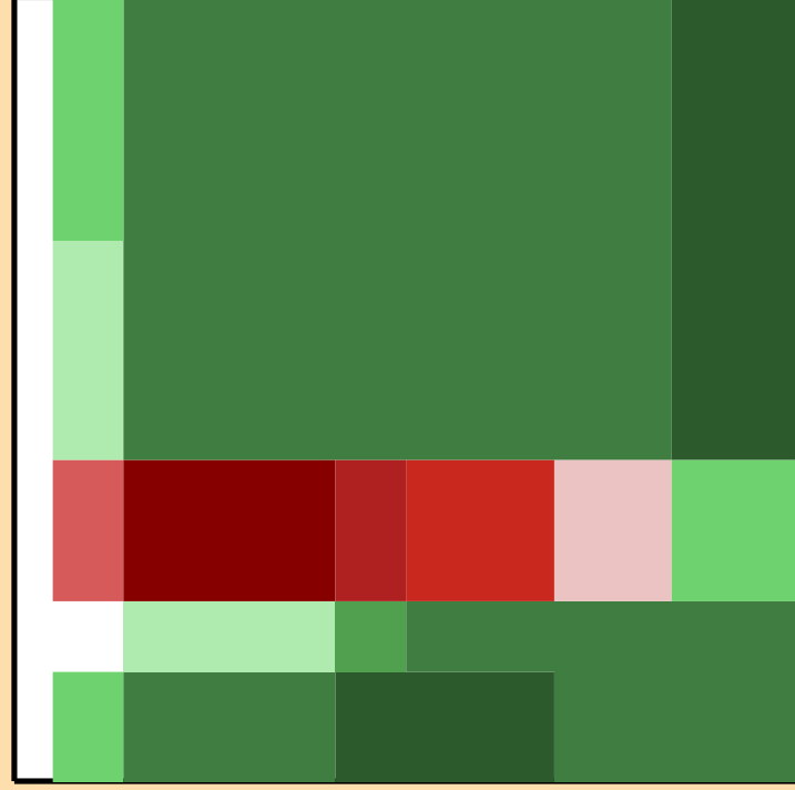
\Delta\sigma/\sigma vs. E for ^{133}\text{Te}(n,2n)
