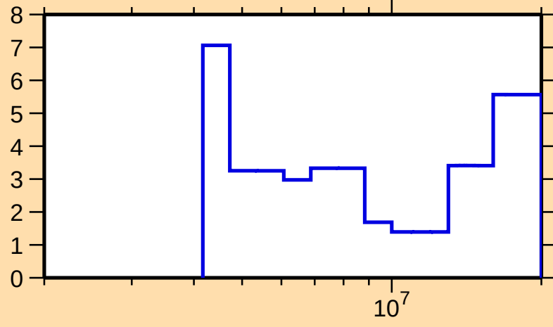
\Delta\sigma/\sigma vs. E for ^{133}\text{Te}(n,\text{tot.})
