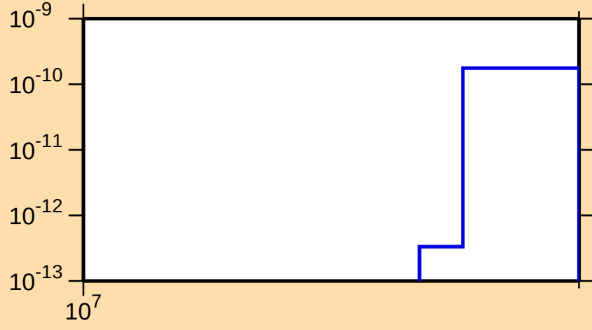
\sigma vs. E for ^{133}\text{Te}(n,2n\alpha)
