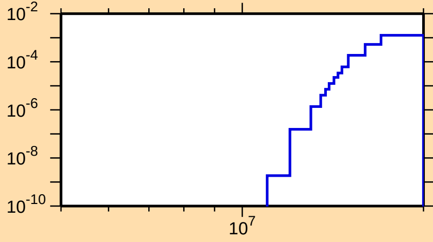
\sigma vs. E for ^{133}\text{Te}(n,d)
