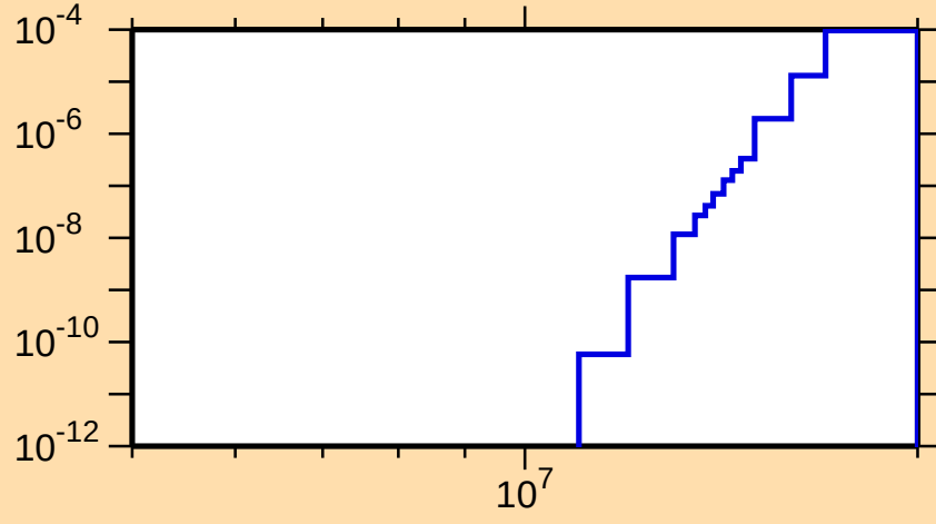
\sigma vs. E for ^{133}\text{Te}(n,n\alpha)
