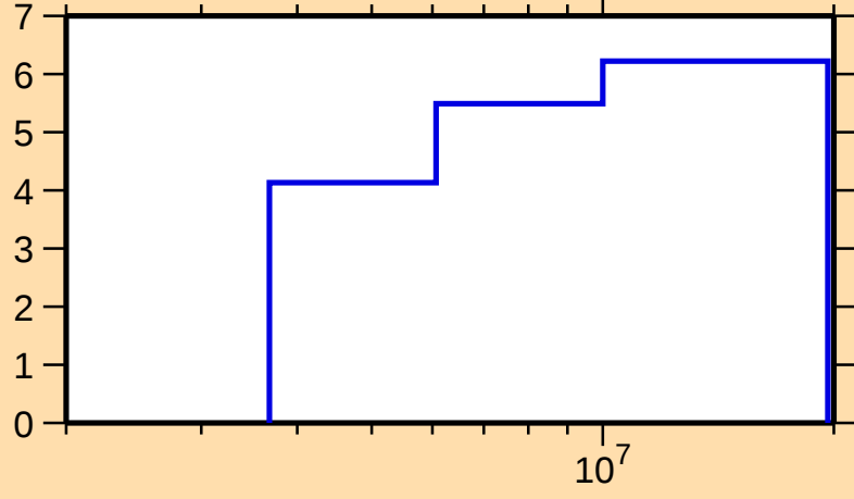
\Delta\sigma/\sigma vs. E for ^{133}\text{Te}(n,n\text{onel.})
