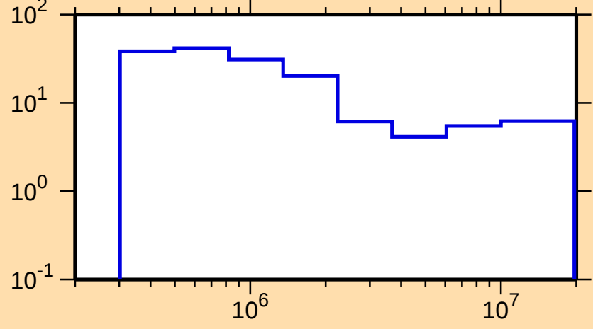
\Delta\sigma/\sigma vs. E for ^{133}\text{Te}(n,\text{nonel.})
