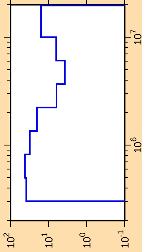
\Delta\sigma/\sigma vs. E for ^{133}\text{Te}(n,\text{inel.})
