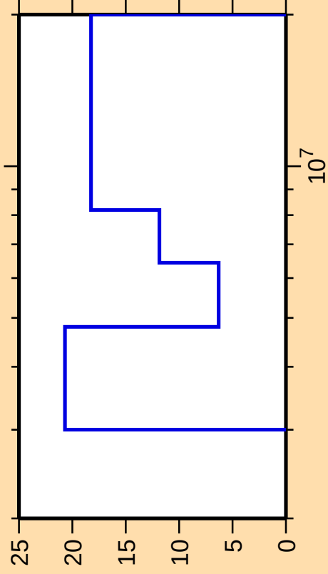
\Delta\sigma/\sigma vs. E for ^{133}\text{Te}(n,\text{ncont.})
