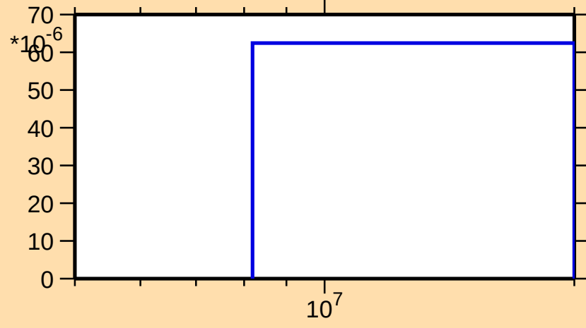
\sigma vs. E for ^{133}\text{Te}(n,d)
