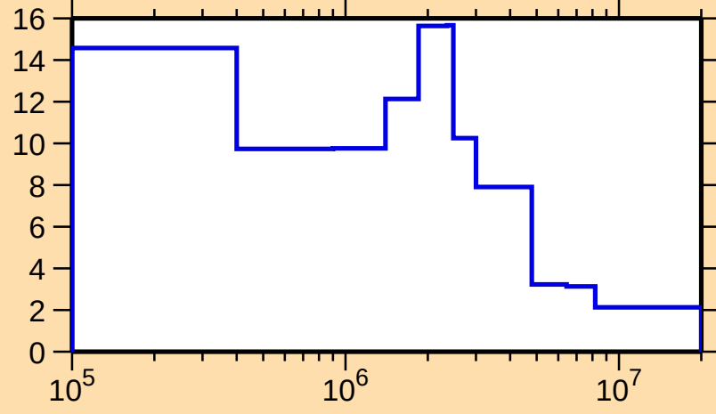
\Delta\sigma/\sigma vs. E for ^{133}\text{Te}(n,\text{tot.})
