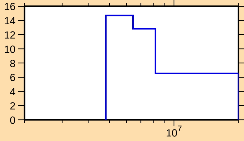
\Delta\sigma/\sigma vs. E for ^{133}\text{Te}(n,2n)
