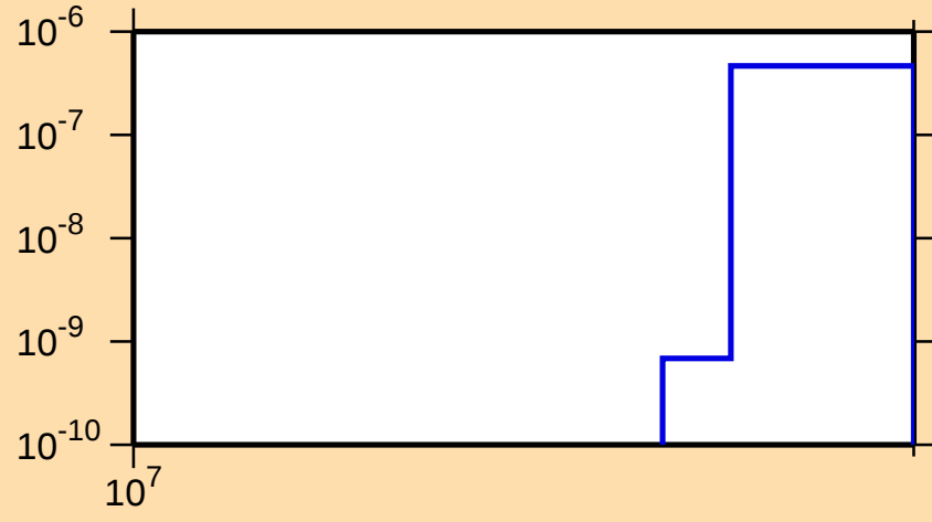
\sigma vs. E for ^{133}\text{Te}(n,\text{nd})
