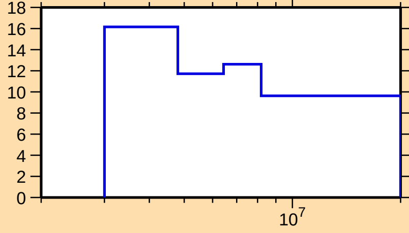
\Delta\sigma/\sigma vs. E for ^{133}\text{Te}(n,\text{nonel.})
