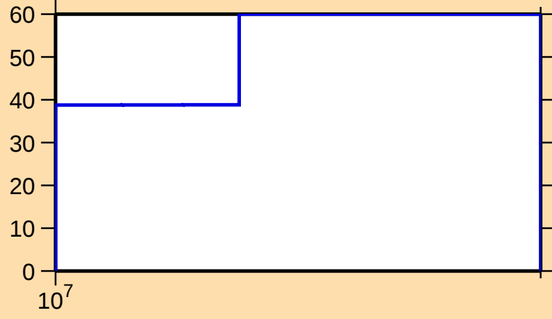
\Delta\sigma/\sigma vs. E for ^{136}\text{Te}(n,2n)
