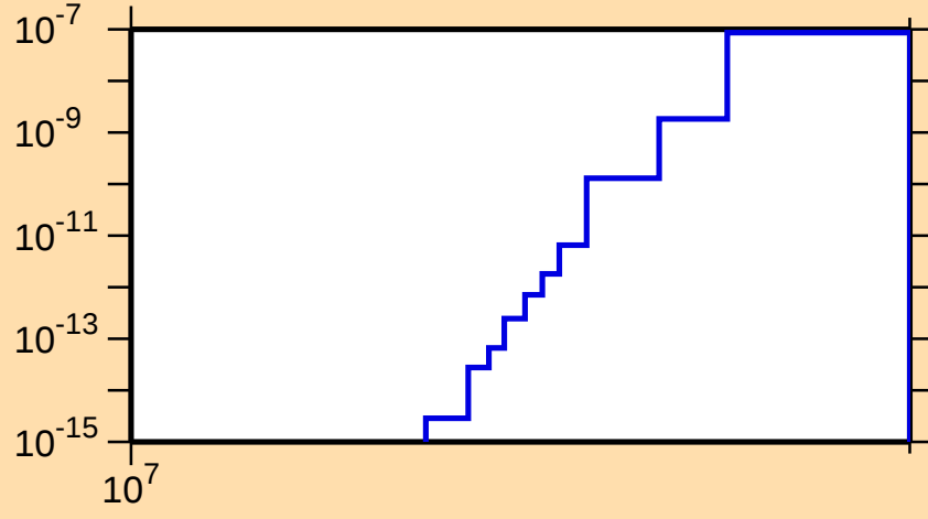
\sigma vs. E for ^{136}\text{Te}(n,2n\alpha)
