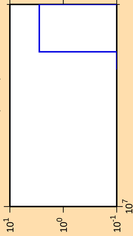
\Delta\sigma/\sigma vs. E for ^{136}\text{Te}(\text{mt } 11)
