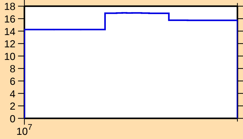
\Delta\sigma/\sigma vs. E for ^{136}\text{Te}(n,\text{nonel.})
