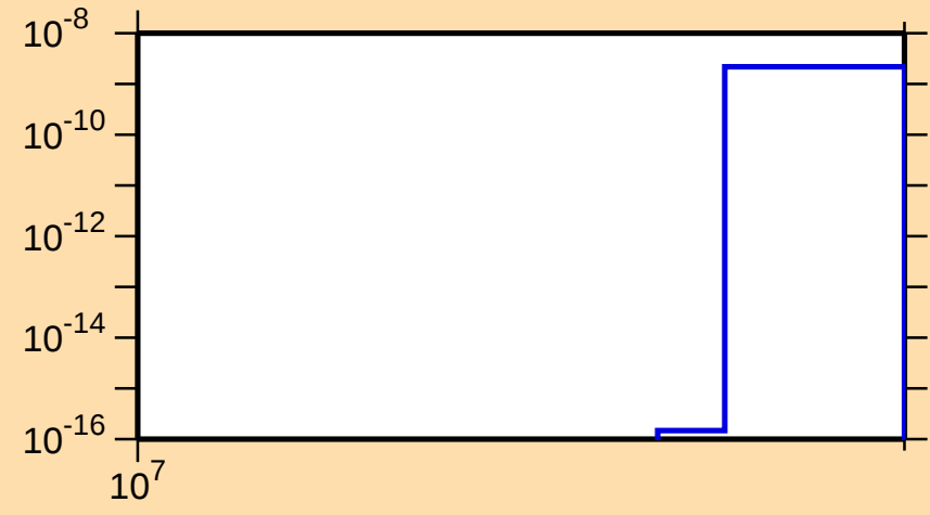
\sigma vs. E for ^{136}\text{Te}(n,2np)
