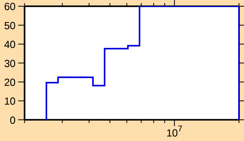
\Delta\sigma/\sigma vs. E for ^{136}\text{Te}(n,\text{inel.})
