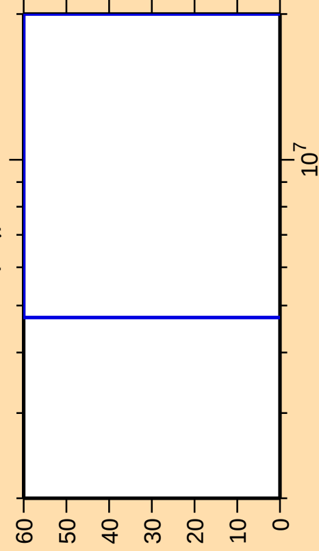
\Delta\sigma/\sigma vs. E for ^{136}\text{Te}(n,\gamma)
