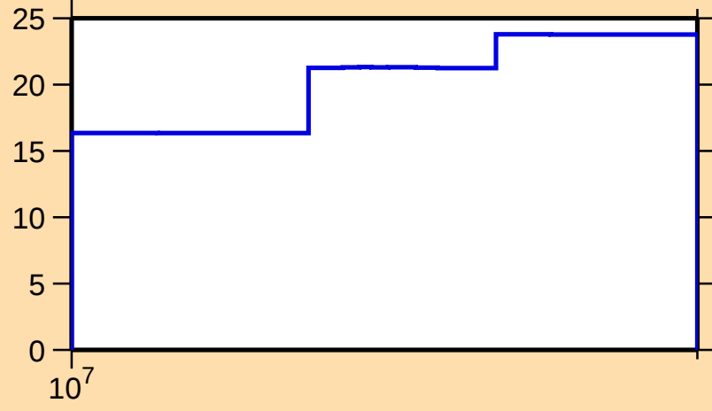
\Delta\sigma/\sigma vs. E for ^{136}\text{Te}(n,\text{tot.})
