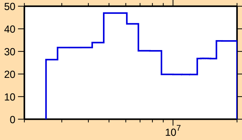
\Delta\sigma/\sigma vs. E for ^{136}\text{Te}(n,\text{el.})
