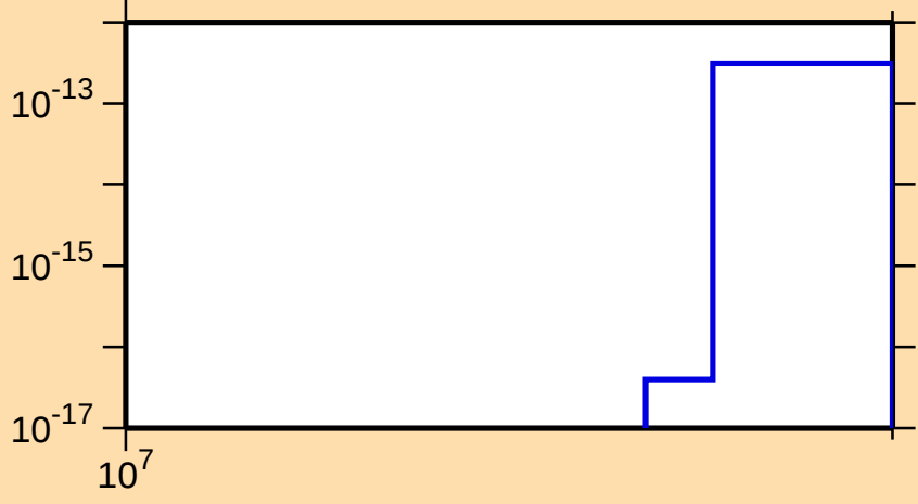
\sigma vs. E for ^{136}\text{Te}(\text{mt } 11)
