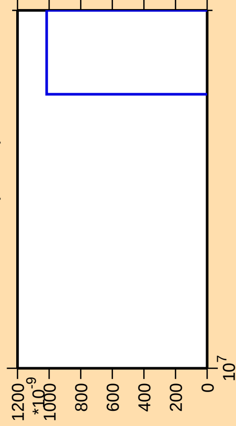
\Delta\sigma/\sigma vs. E for ^{136}\text{Te}(\text{mt } 42)
