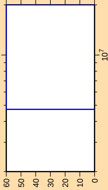
\Delta\sigma/\sigma vs. E for ^{136}\text{Te}(n,n_{\text{cont}})
