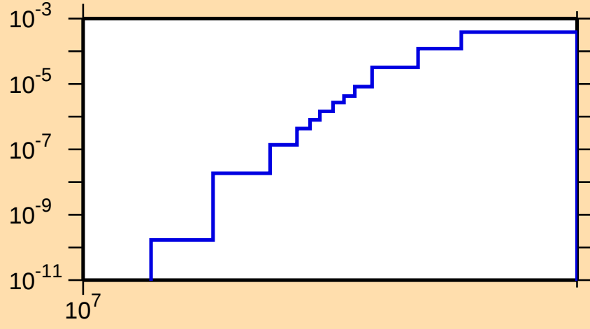
\sigma vs. E for ^{136}\text{Te}(n,p)
