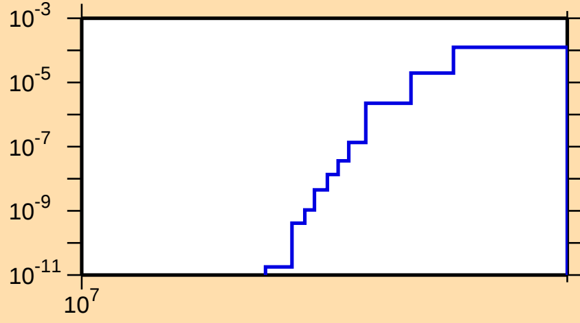
\sigma vs. E for ^{136}\text{Te}(n,nt)
