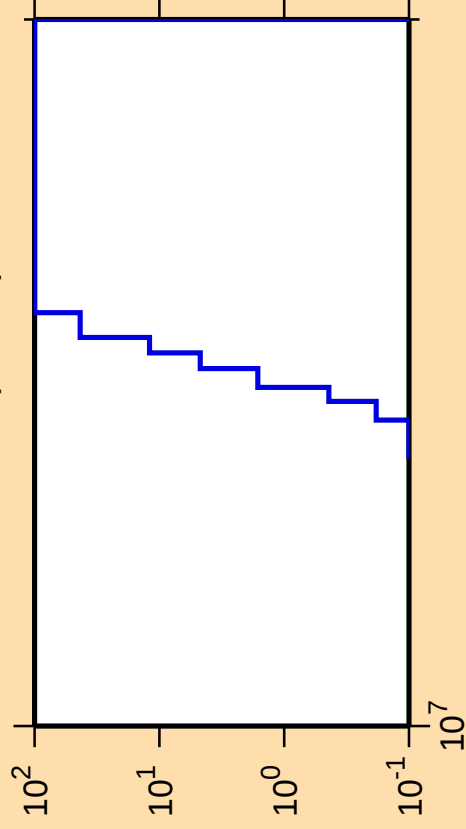
\Delta\sigma/\sigma vs. E for ^{136}\text{Te}(n,2n\alpha)
