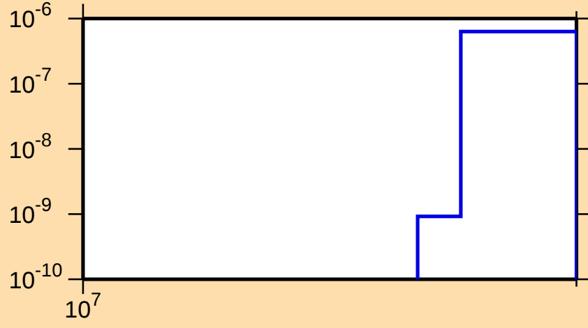
\sigma vs. E for ^{136}\text{Te}(n,\text{nd})
