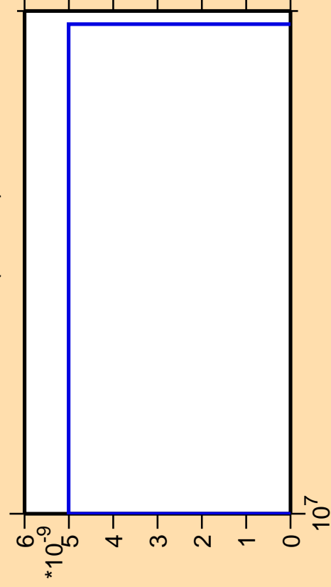
\Delta\sigma/\sigma vs. E for ^{136}\text{Te} (mt 42)
