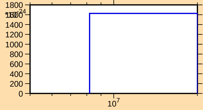
\sigma vs. E for ^{136}\text{Te}(\text{mt } 42)
