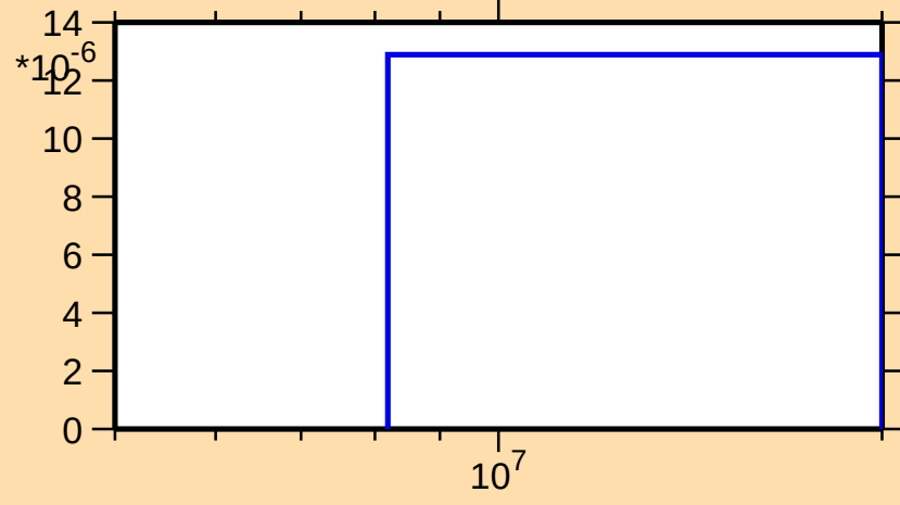
\sigma vs. E for ^{136}\text{Te}(n,p)
