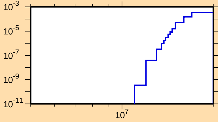
\sigma vs. E for ^{138}\text{Te}(n,t)
