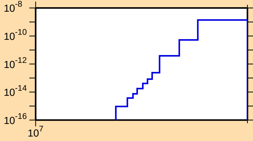
\sigma vs. E for ^{138}\text{Te}(n,3n\alpha)
