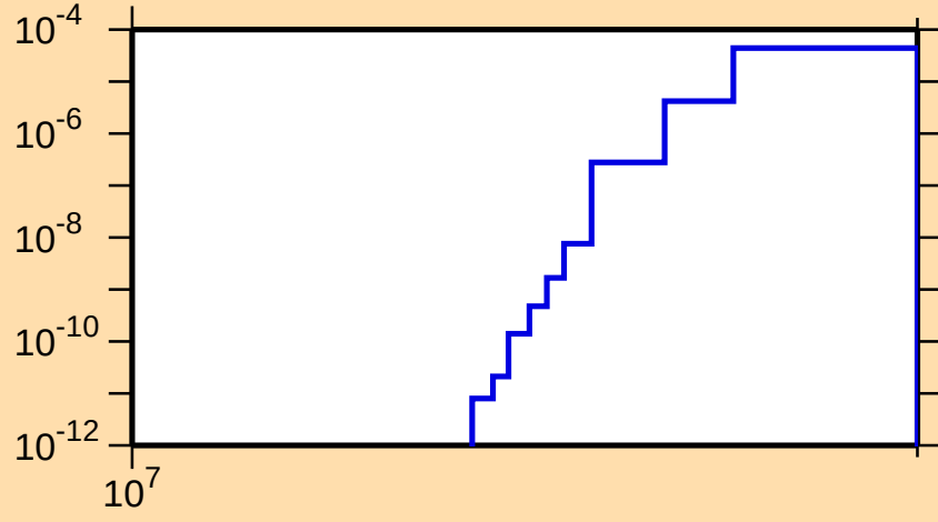
\sigma vs. E for ^{138}\text{Te}(n,nt)
