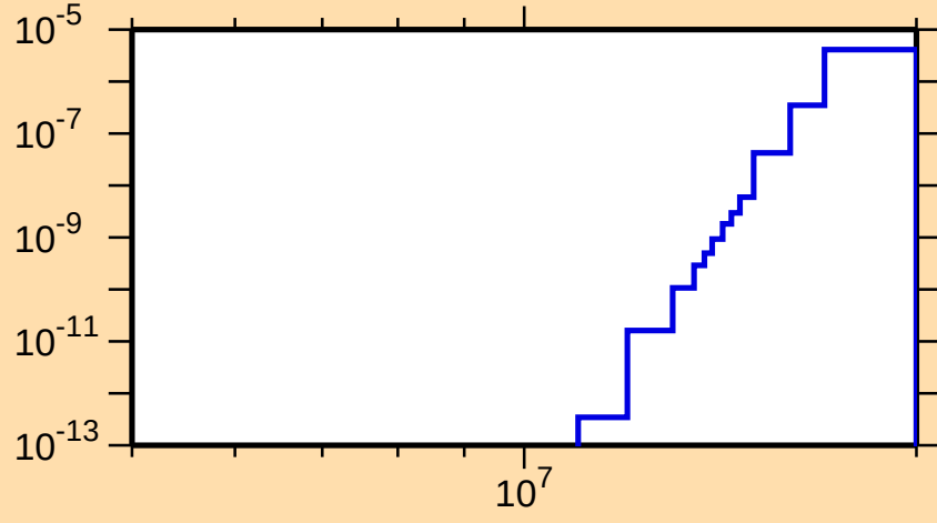
\sigma vs. E for ^{138}\text{Te}(n,2n\alpha)
