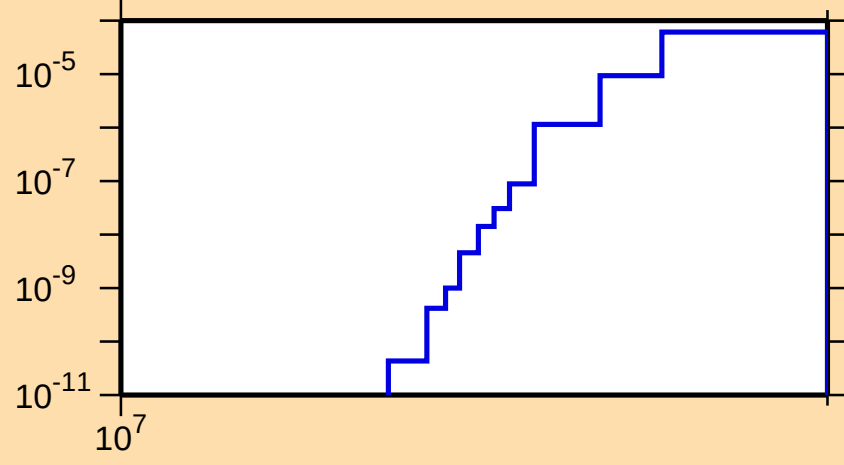
\sigma vs. E for ^{138}\text{Te}(n,p)
