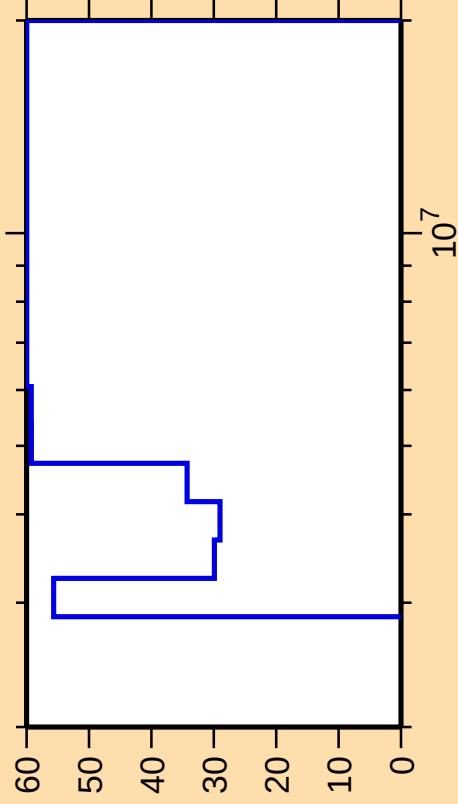
\Delta\sigma/\sigma vs. E for ^{138}\text{Te}(n,n\text{cont.})
