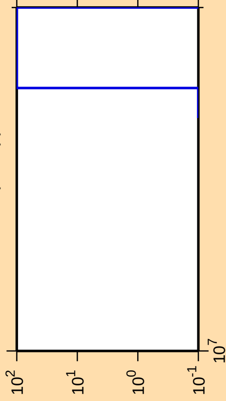
\Delta\sigma/\sigma vs. E for ^{138}\text{Te}(n,2np)
