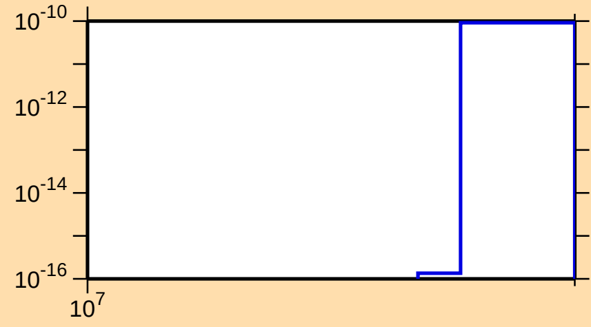
\sigma vs. E for ^{138}\text{Te}(n,2np)
