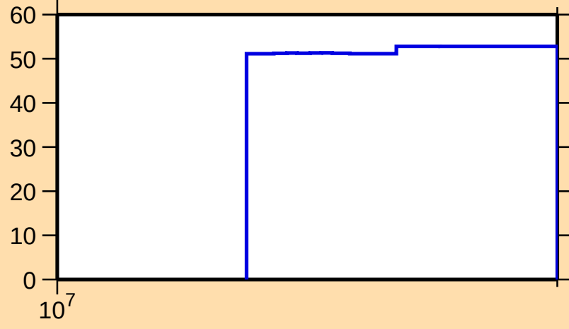
\Delta\sigma/\sigma vs. E for ^{138}\text{Te}(n,2n)
