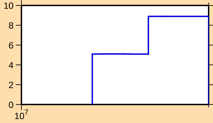
\Delta\sigma/\sigma vs. E for ^{138}\text{Te}(n,\text{el.})
