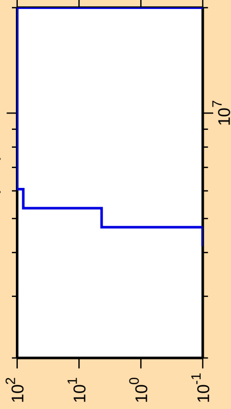
\Delta\sigma/\sigma vs. E for ^{138}\text{Te}(n,\alpha)
