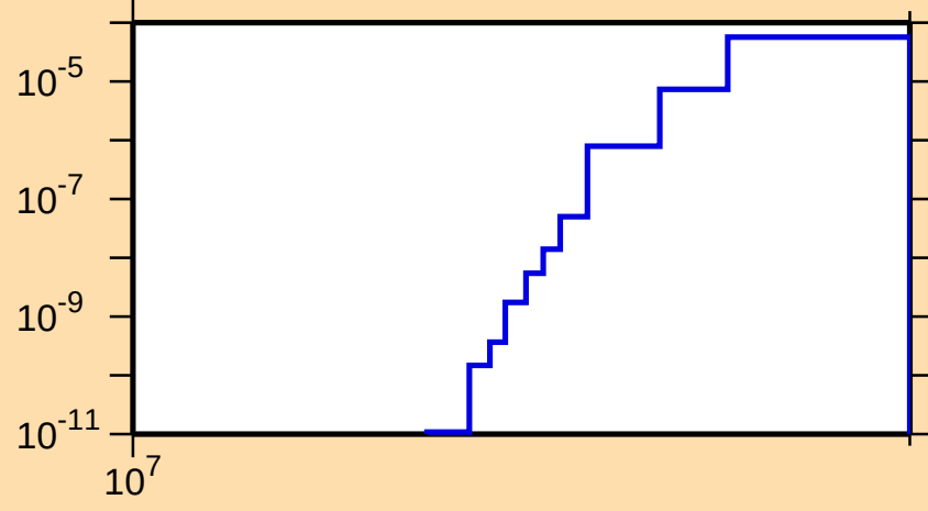
\sigma vs. E for ^{138}\text{Te}(n,d)
