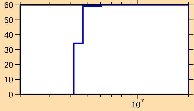
\Delta\sigma/\sigma vs. E for ^{138}\text{Te}(n,n\text{cont.})
