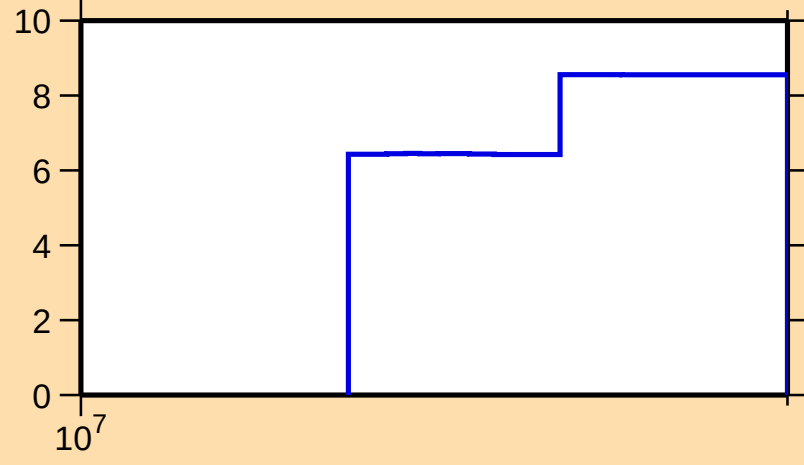
\Delta\sigma/\sigma vs. E for ^{138}\text{Te}(n,\text{tot.})
