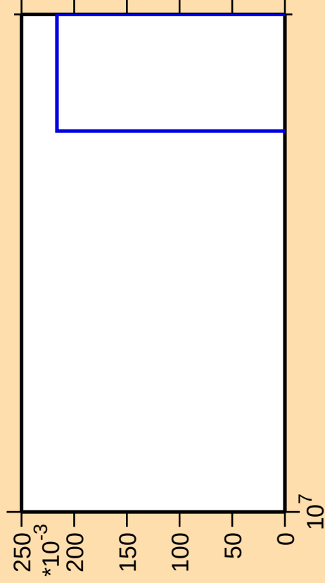
\Delta\sigma/\sigma vs. E for ^{138}\text{Te}(\text{mt } 11)
