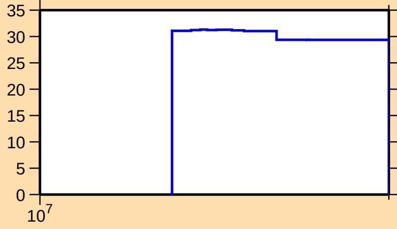
\Delta\sigma/\sigma vs. E for ^{138}\text{Te}(n,n_1)
