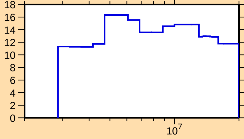
\Delta\sigma/\sigma vs. E for ^{138}\text{Te}(n,\text{nonel.})
