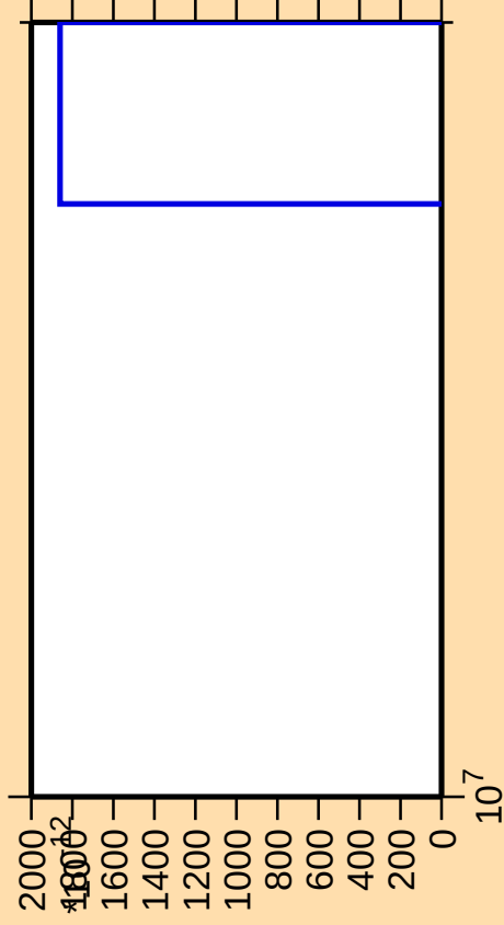
\Delta\sigma/\sigma vs. E for ^{138}\text{Te}(\text{mt } 42)
