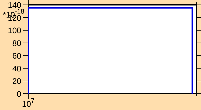
\sigma vs. E for ^{138}\text{Te}(\text{mt } 11)
