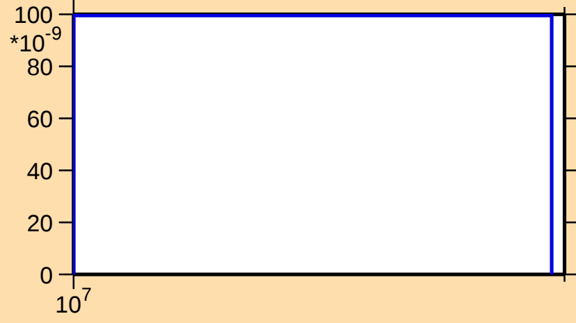
\sigma vs. E for ^{138}\text{Te}(n,np)
