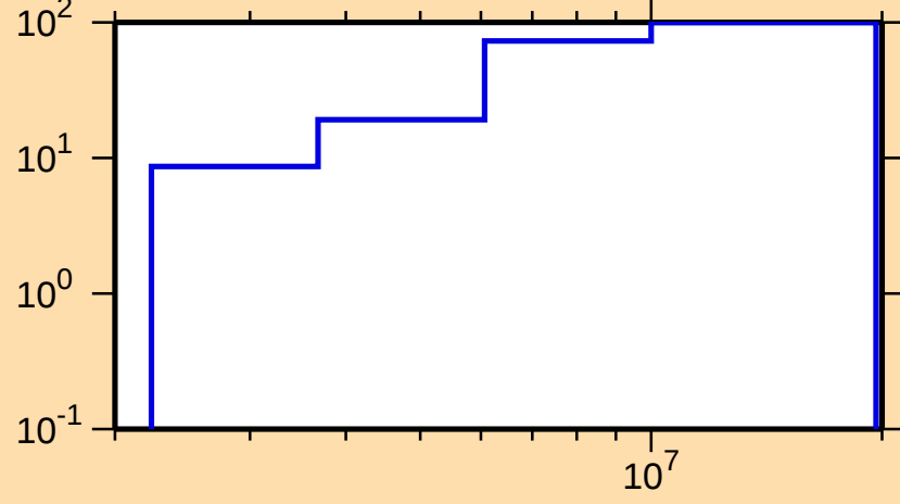
\Delta\sigma/\sigma vs. E for ^{138}\text{Te}(n,\text{inel.})
