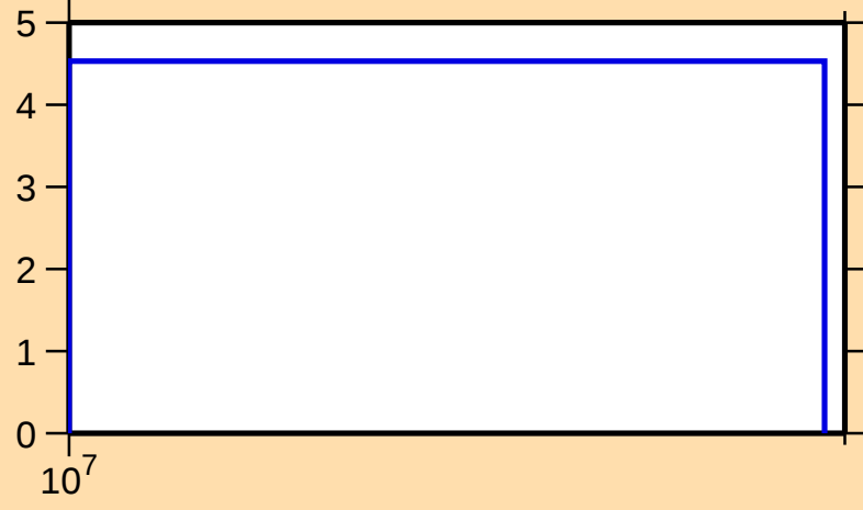
\Delta\sigma/\sigma vs. E for ^{138}\text{Te}(n,\text{el.})
