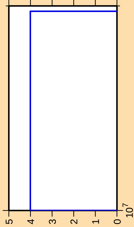
\Delta\sigma/\sigma vs. E for ^{138}\text{Te}(n,2np)
