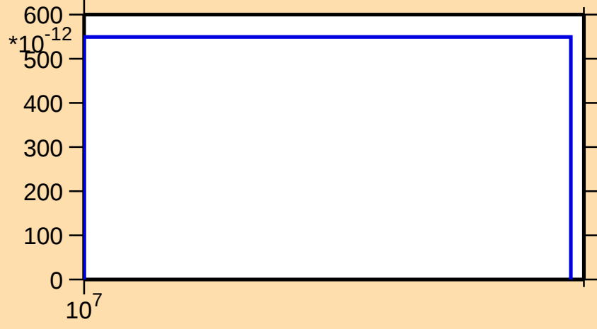
\sigma vs. E for ^{138}\text{Te}(n,\text{nd})
