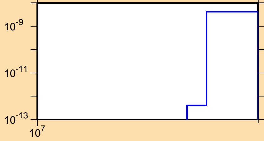
\sigma vs. E for ^{45}\text{Ti}(\text{mt117})
