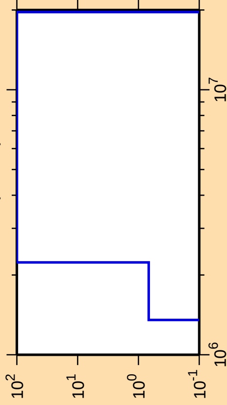
\Delta\sigma/\sigma vs. E for ^{180}\text{Tl}(\text{mt } 45)
