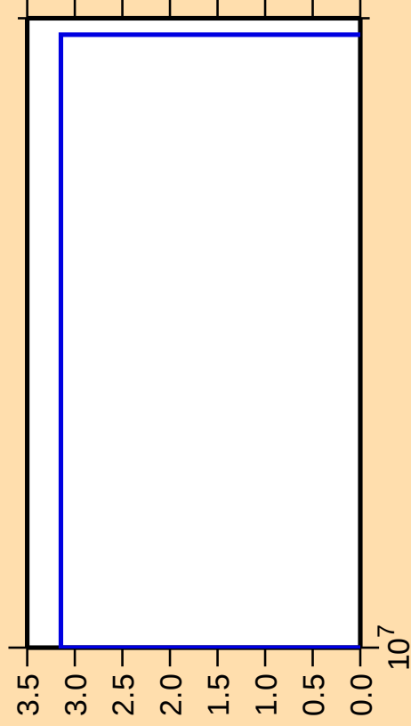
\Delta\sigma/\sigma vs. E for ^{180}\text{Tl}(n,\text{nt})
