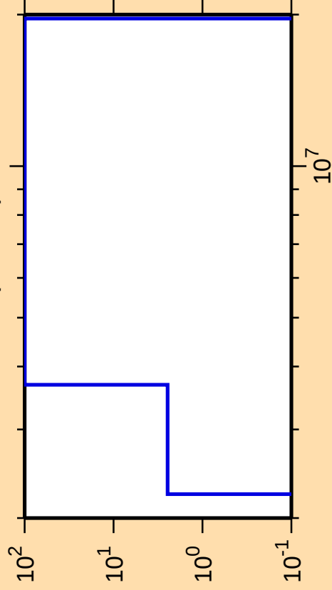
\Delta\sigma/\sigma vs. E for ^{180}\text{Tl}(\text{mt117})
