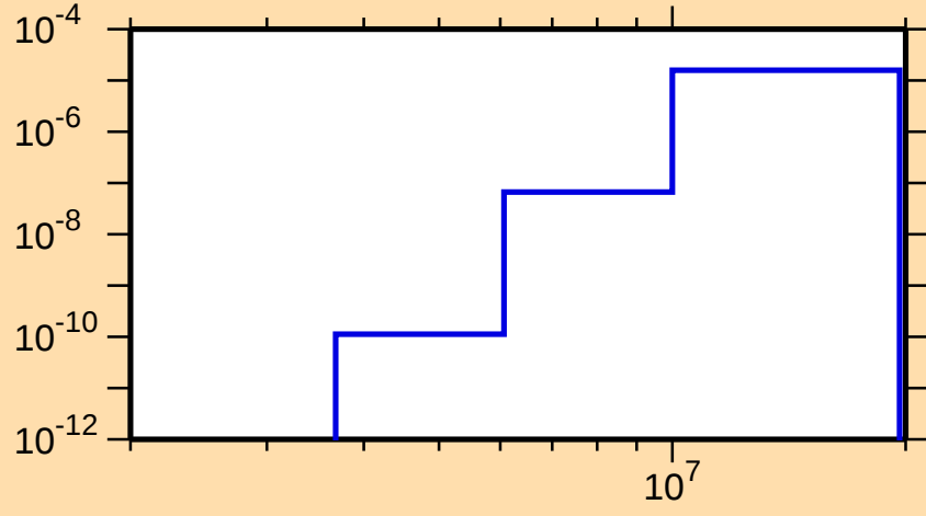
\sigma vs. E for ^{180}\text{Tl}(\text{mt117})
