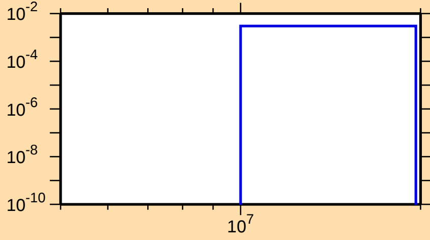
\sigma vs. E for ^{180}\text{Tl}(n,2np)
