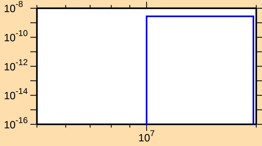
\sigma vs. E for ^{180}\text{Tl}(\text{mt } 34)
