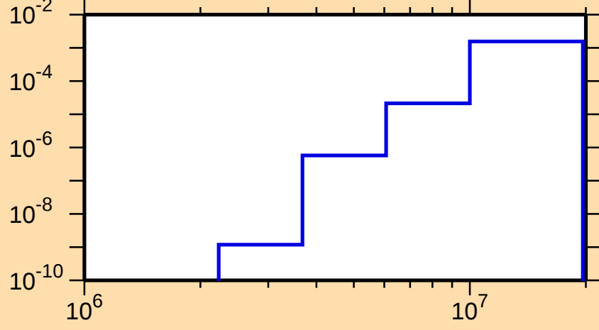
\sigma vs. E for ^{180}\text{Tl}(\text{mt } 45)
