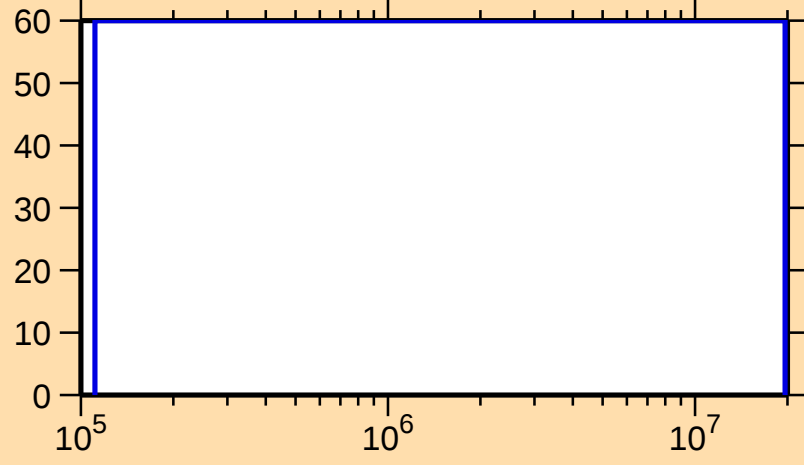
\Delta\sigma/\sigma vs. E for ^{180}\text{Tl}(n,ncont.)
