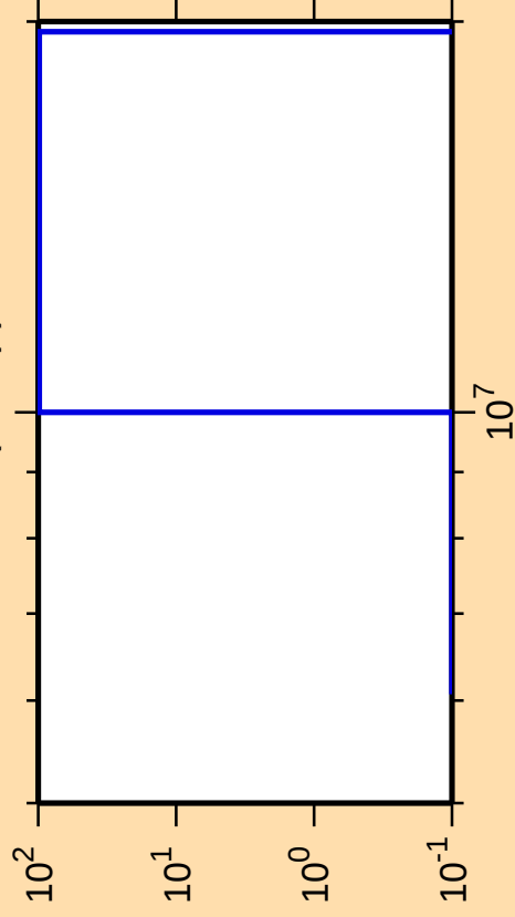
\Delta\sigma/\sigma vs. E for ^{180}\text{Tl}(n,2np)
