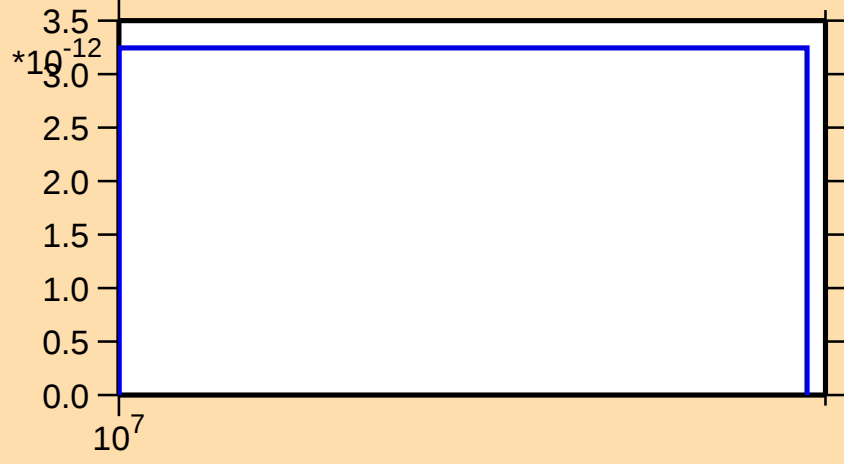
\sigma vs. E for ^{180}\text{Tl}(n,\text{nt})
