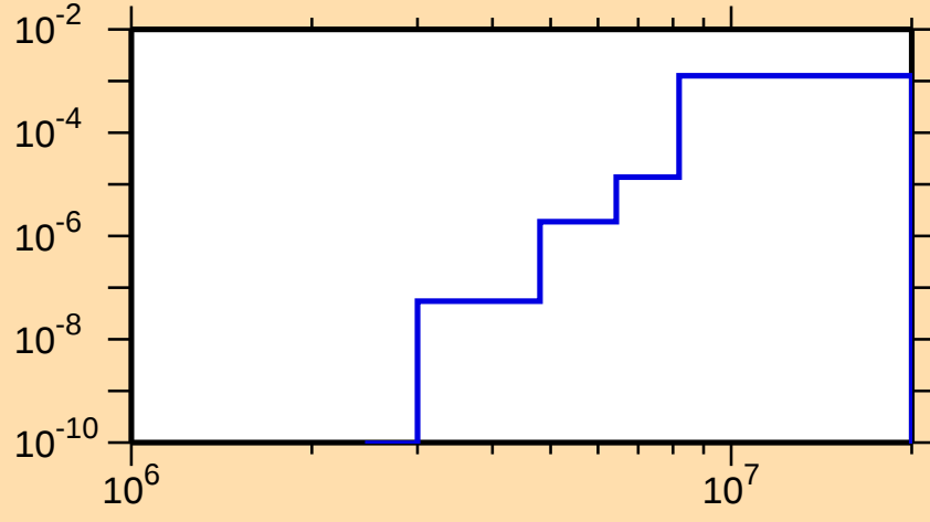
\sigma vs. E for ^{180}\text{Tl}(\text{mt 45})
