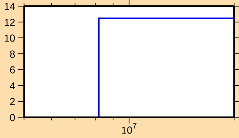
\Delta\sigma/\sigma vs. E for ^{180}\text{Tl}(n,\text{nonel.})
