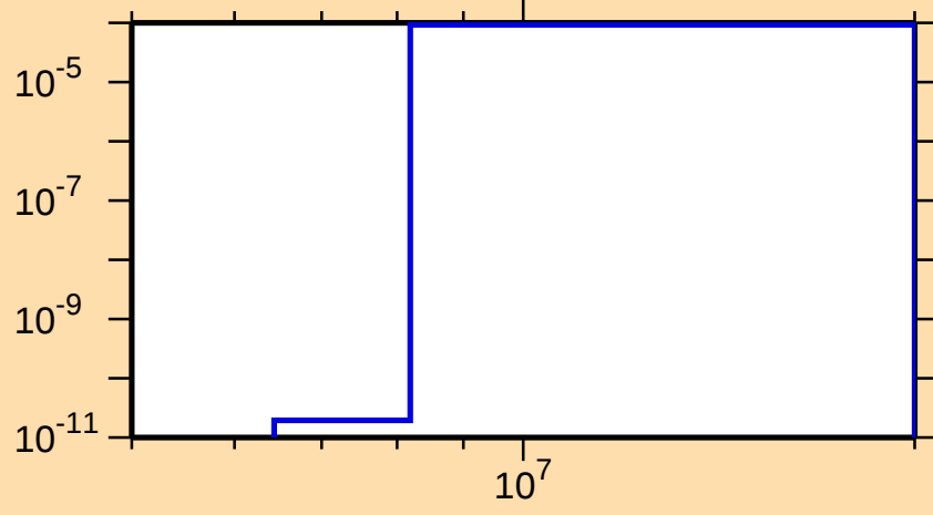
\sigma vs. E for ^{180}\text{Tl}(n,\text{pd})
