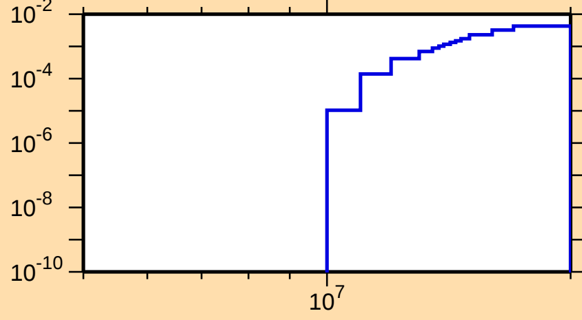
\sigma vs. E for ^{182}\text{Tl}(n,2n\alpha)
