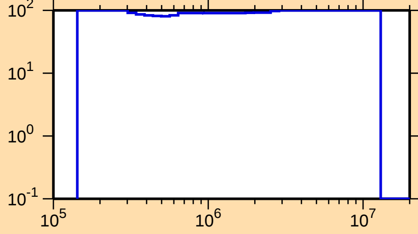
\Delta\sigma/\sigma vs. E for ^{182}\text{Tl}(n,n_1)
