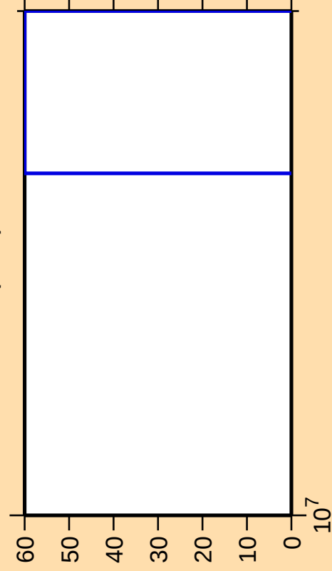
\Delta\sigma/\sigma vs. E for ^{182}\text{Tl}(n,\text{nt})
