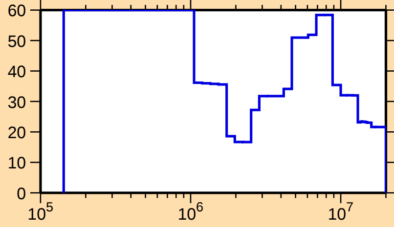
\Delta\sigma/\sigma vs. E for ^{182}\text{Tl}(n,\text{el.})
