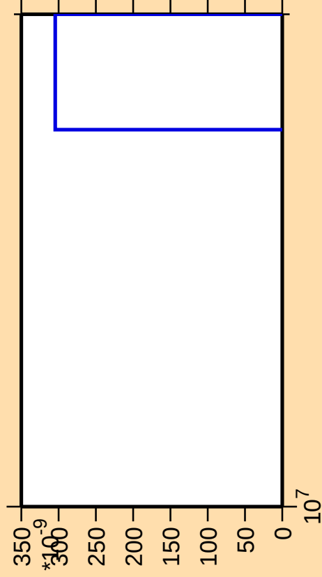
\Delta\sigma/\sigma vs. E for ^{182}\text{Tl}(\text{mt 42})
