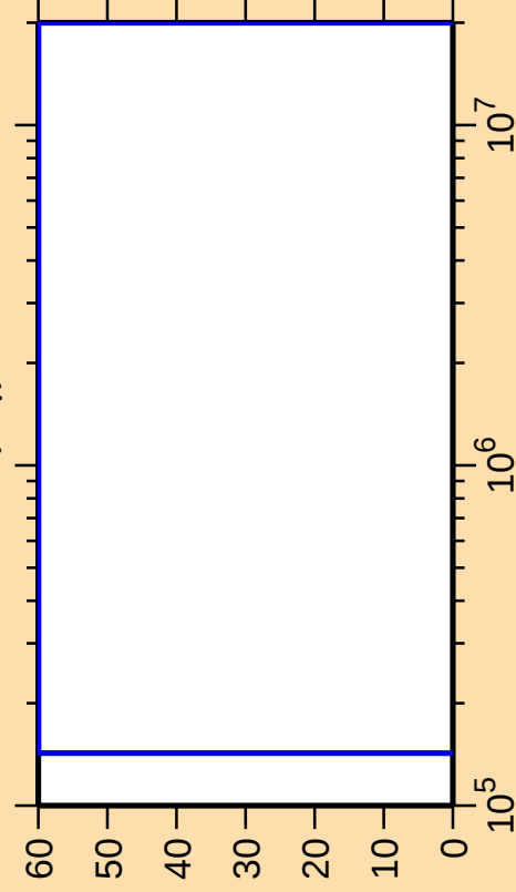
\Delta\sigma/\sigma vs. E for ^{182}\text{Tl}(n,\gamma)
