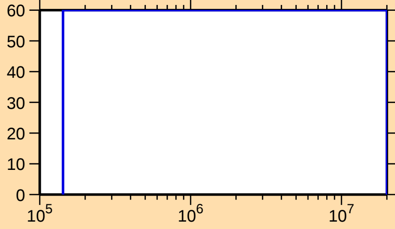
\Delta\sigma/\sigma vs. E for ^{182}\text{Tl}(n,n\text{cont.})
