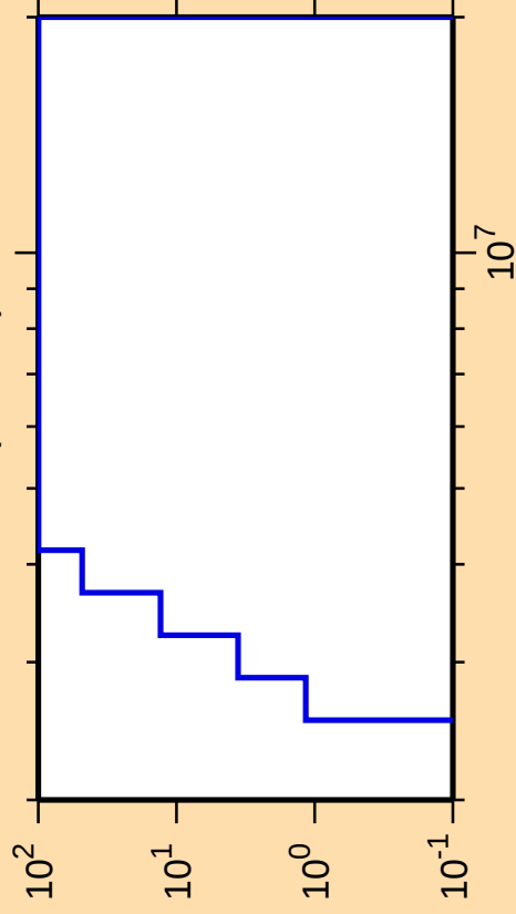
\Delta\sigma/\sigma vs. E for ^{182}\text{Tl}(n,\text{He3})
