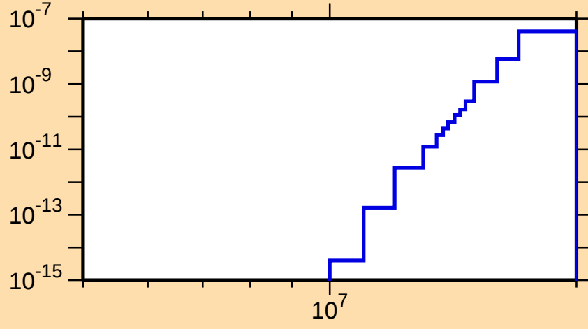
\sigma vs. E for ^{182}\text{Tl}(\text{mt } 34)
