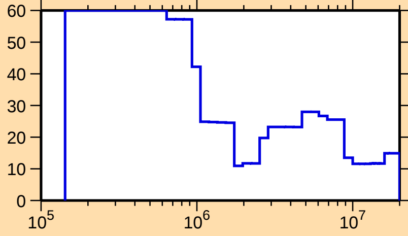
\Delta\sigma/\sigma vs. E for ^{182}\text{Tl}(n,\text{tot.})
