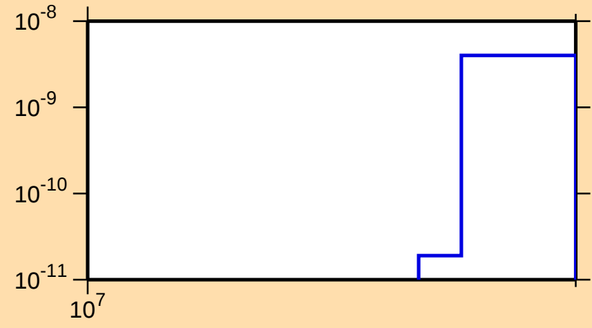
\sigma vs. E for ^{182}\text{Tl}(n,\text{nt})
