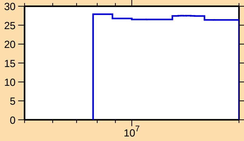
\Delta\sigma/\sigma vs. E for ^{182}\text{Tl}(n,\text{nonel.})
