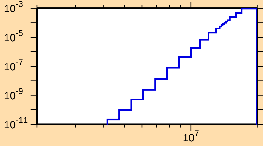
\sigma vs. E for ^{182}\text{Tl}(n,\text{He3})
