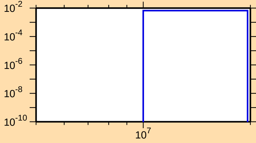
\sigma vs. E for ^{182}\text{Tl}(n,2np)
