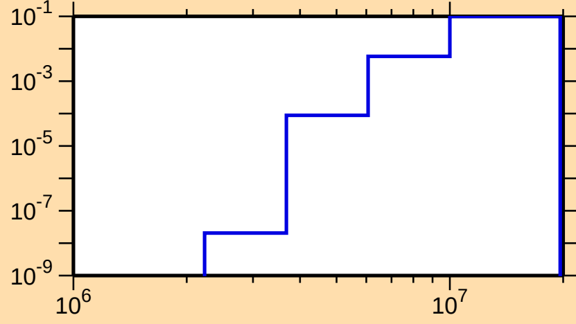
\sigma vs. E for ^{182}\text{Tl}(\text{mt } 45)
