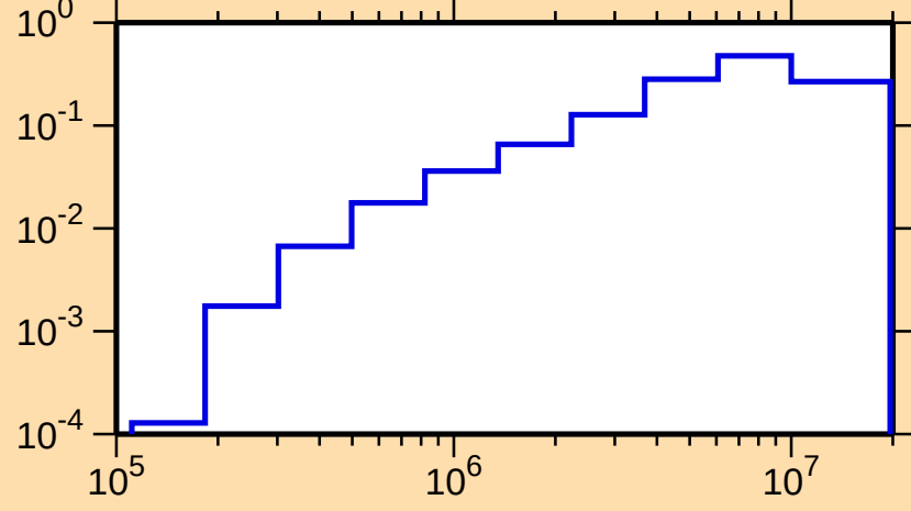
\sigma vs. E for ^{182}\text{Tl}(n,\text{inel.})
