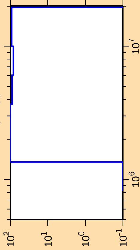
\Delta\sigma/\sigma vs. E for ^{182}\text{Tl}(n,np)
