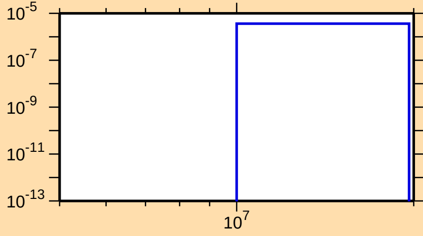
\sigma vs. E for ^{182}\text{Tl}(n,\text{nd})
