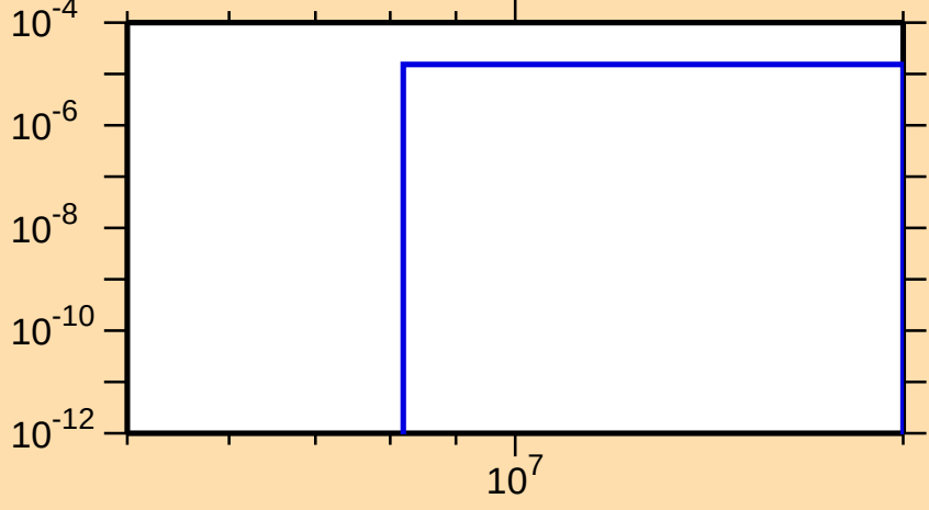
\sigma vs. E for ^{182}\text{Tl}(n,\text{pd})
