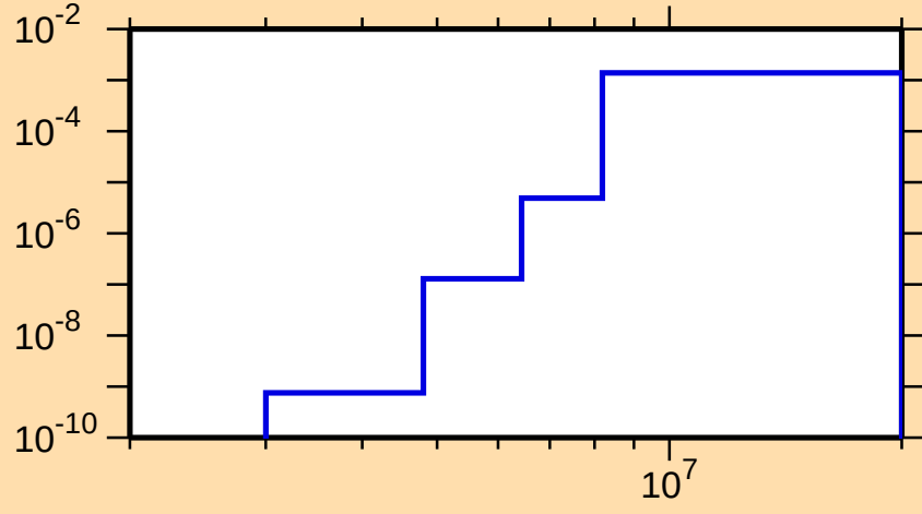
\sigma vs. E for ^{182}\text{Tl}(\text{mt117})
