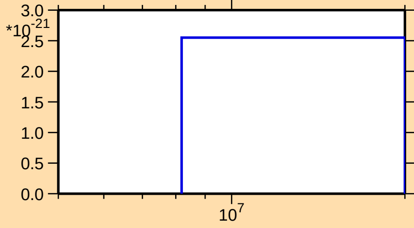
\sigma vs. E for ^{182}\text{Tl}(\text{mt } 42)
