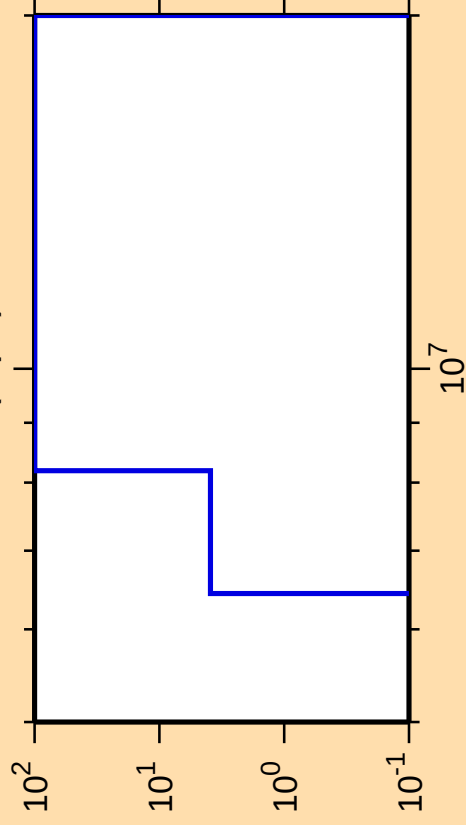
\Delta\sigma/\sigma vs. E for ^{182}\text{Tl}(n,\text{pd})
