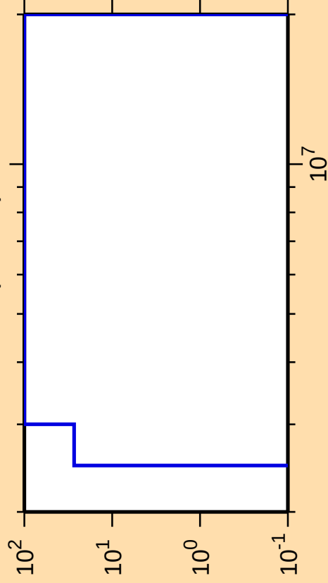
\Delta\sigma/\sigma vs. E for ^{182}\text{Tl}(\text{mt117})
