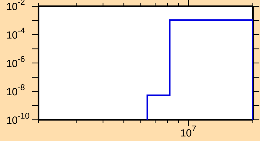
\sigma vs. E for ^{182}\text{Tl}(n,t)
