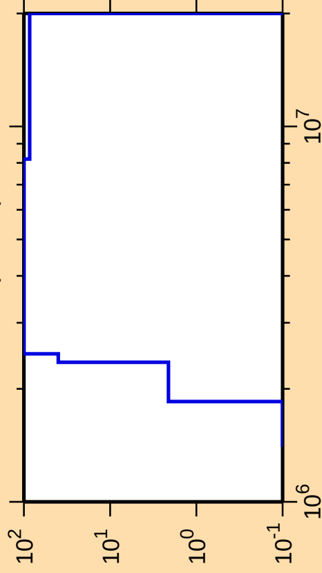
\Delta\sigma/\sigma vs. E for ^{182}\text{Tl}(\text{mt 45})
