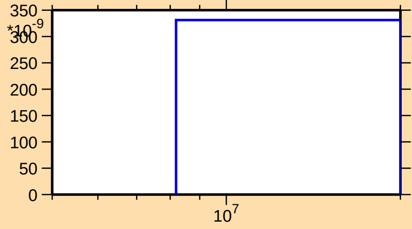
\sigma vs. E for ^{182}\text{Tl}(n,\text{pt})
