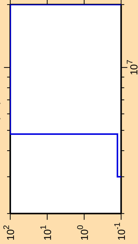
\Delta\sigma/\sigma vs. E for ^{182}\text{Tl}(n,t)
