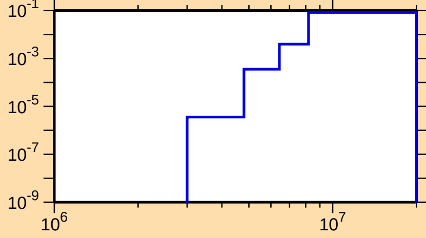
\sigma vs. E for ^{182}\text{Tl}(\text{mt 45})
