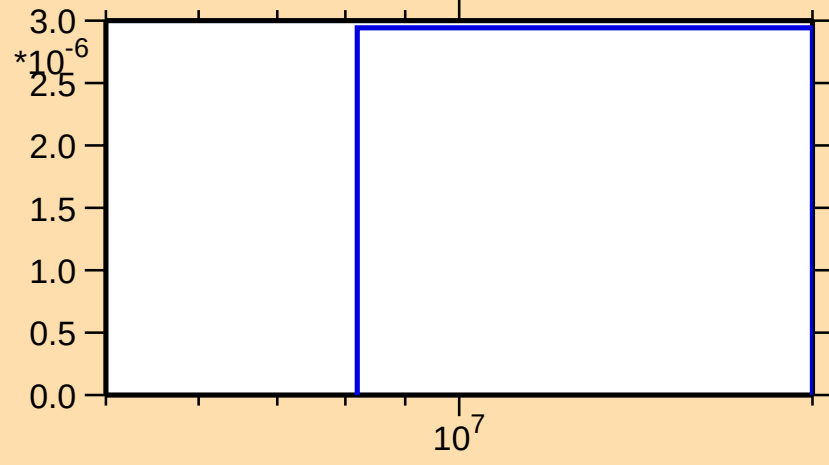
\sigma vs. E for ^{182}\text{Tl}(n,\text{nd})
