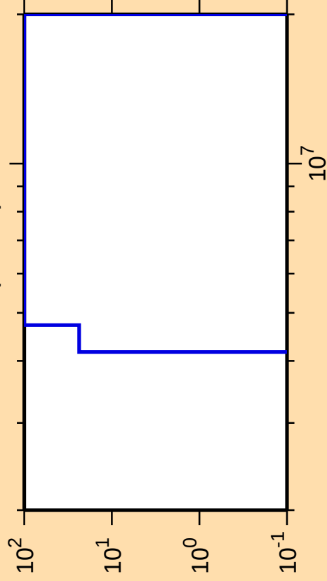
\Delta\sigma/\sigma vs. E for ^{185}\text{Tl}(\text{mt 45})
