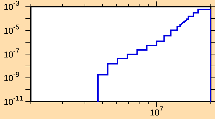
\sigma vs. E for ^{185}\text{Tl}(\text{mt 45})
