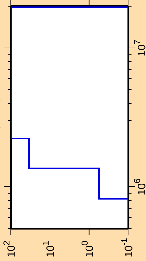
\Delta\sigma/\sigma vs. E for ^{185}\text{Tl}(n,n\alpha)
