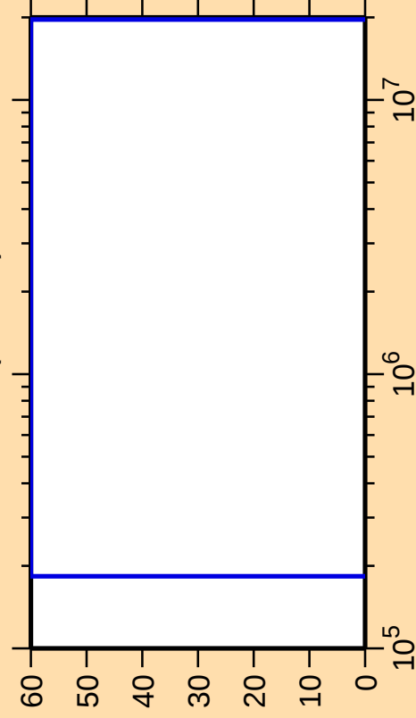
\Delta\sigma/\sigma vs. E for ^{185}\text{Tl}(n,\text{inel.})
