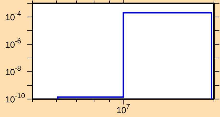
\sigma vs. E for ^{185}\text{Tl}(n,t)
