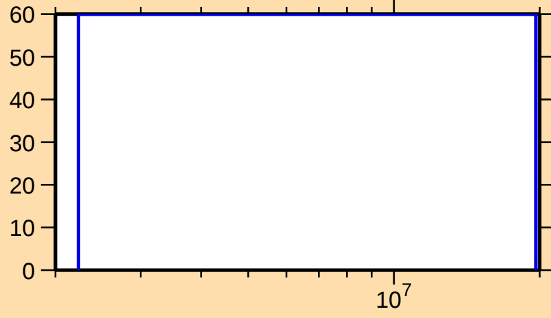
\Delta\sigma/\sigma vs. E for ^{185}\text{Tl}(n,n\text{cont.})
