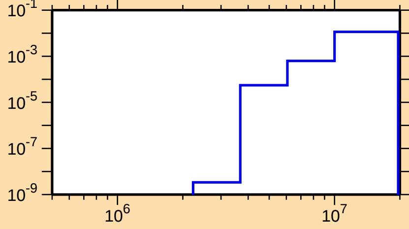
\sigma vs. E for ^{185}\text{Tl}(n,n\alpha)
