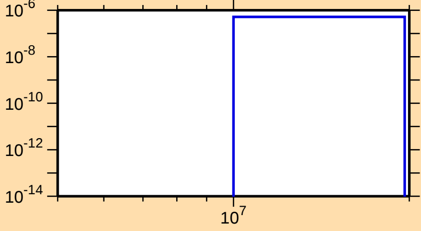
\sigma vs. E for ^{185}\text{Tl}(n,2n\alpha)
