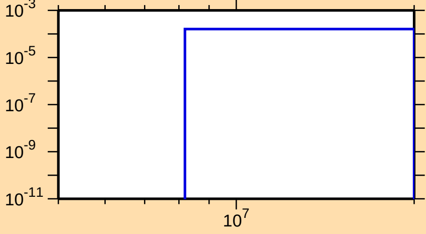
\sigma vs. E for ^{185}\text{Tl}(n,t)
