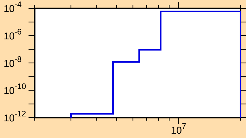
\sigma vs. E for ^{185}\text{Tl}(\text{mt } 45)
