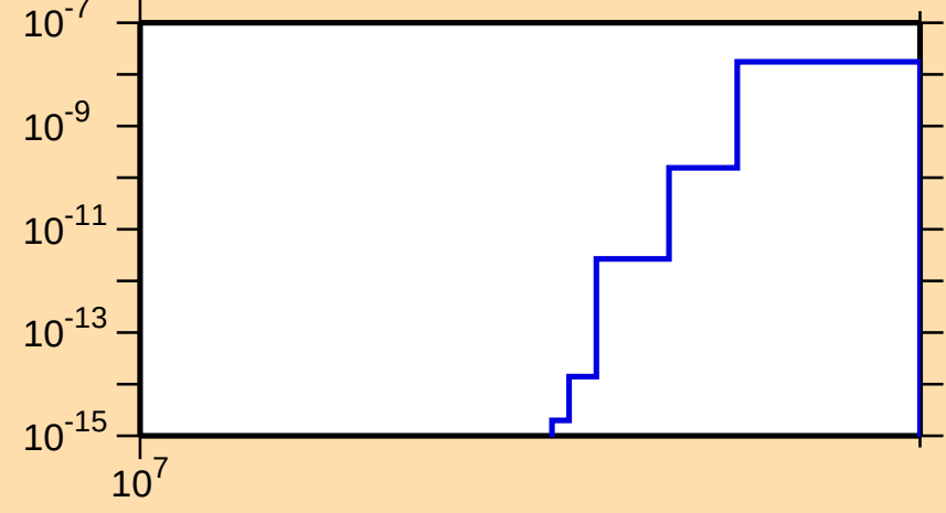
\sigma vs. E for ^{187}\text{Tl}(n,\text{nt})
