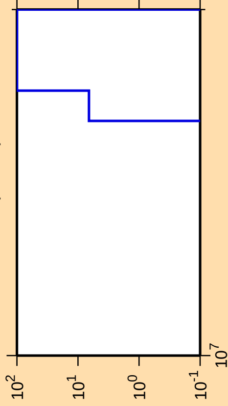
\Delta\sigma/\sigma vs. E for ^{187}\text{Tl}(\text{mt 34})
