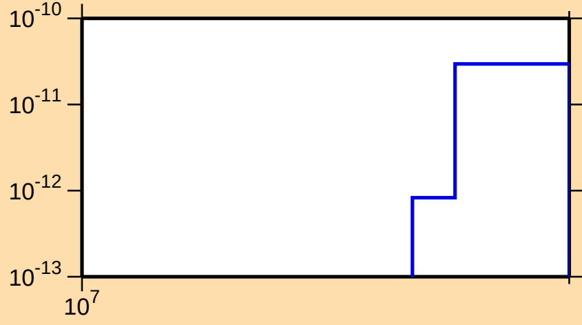
\sigma vs. E for ^{187}\text{Tl}(\text{mt 34})
