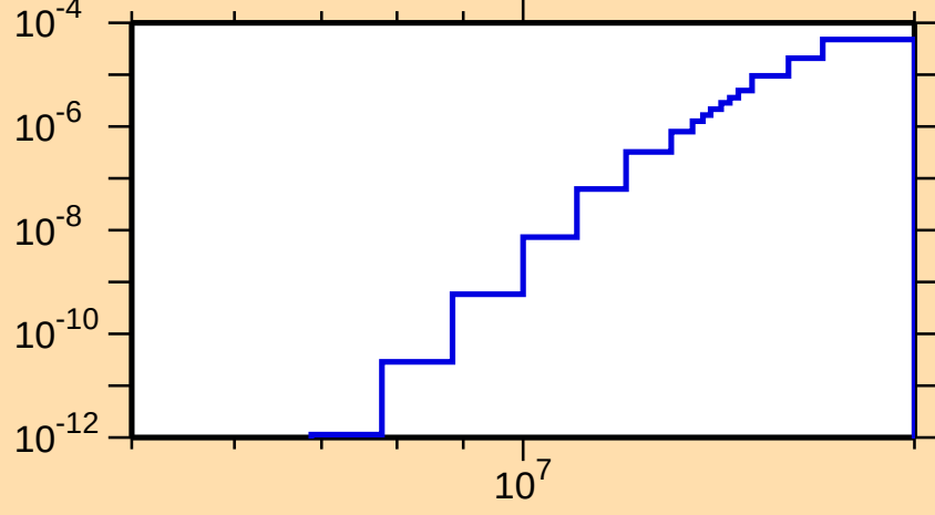
\sigma vs. E for ^{187}\text{Tl}(\text{mt } 45)
