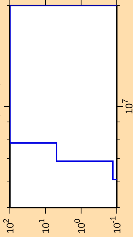
\Delta\sigma/\sigma vs. E for ^{187}\text{Tl}(\text{mt } 45)
