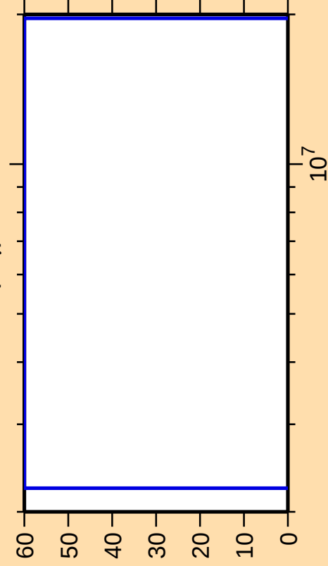
\Delta\sigma/\sigma vs. E for ^{187}\text{Tl}(n,\gamma)
