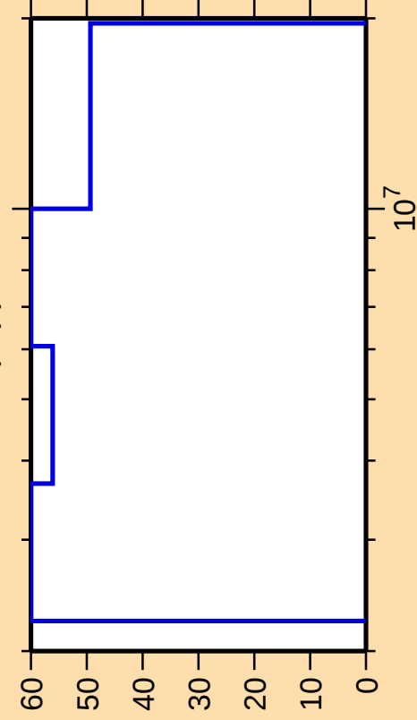
\Delta\sigma/\sigma vs. E for ^{187}\text{Tl}(n,p)
