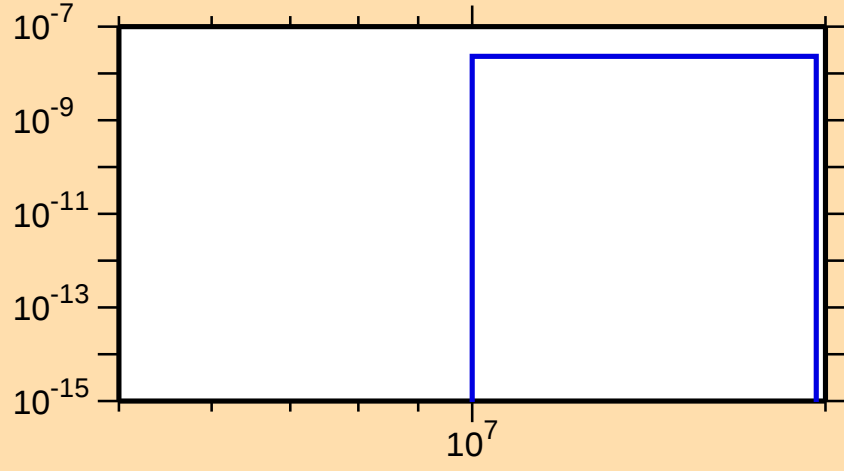
\sigma vs. E for ^{187}\text{Tl}(n,\text{pd})
