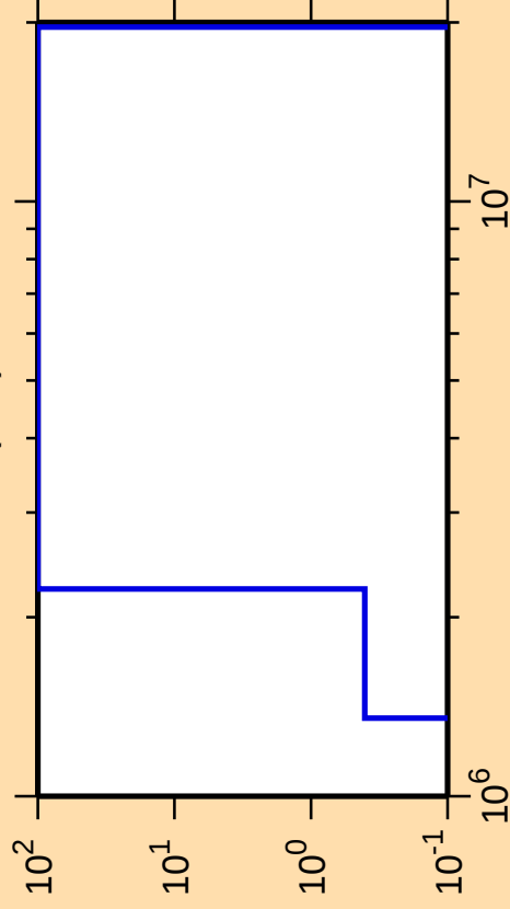
\Delta\sigma/\sigma vs. E for ^{187}\text{Tl}(n,d)
