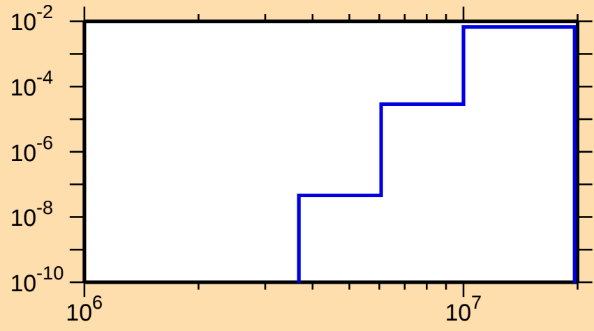
\sigma vs. E for ^{187}\text{Tl}(n,d)
