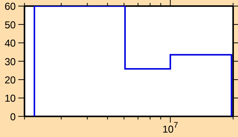
\Delta\sigma/\sigma vs. E for ^{187}\text{Tl}(n,ncont.)
