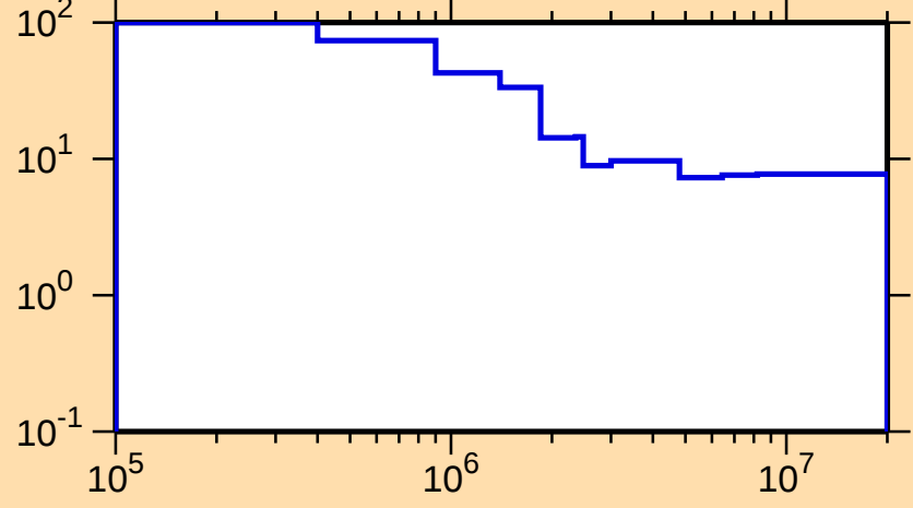
\Delta\sigma/\sigma vs. E for ^{187}\text{Tl}(n,\text{nonel.})
