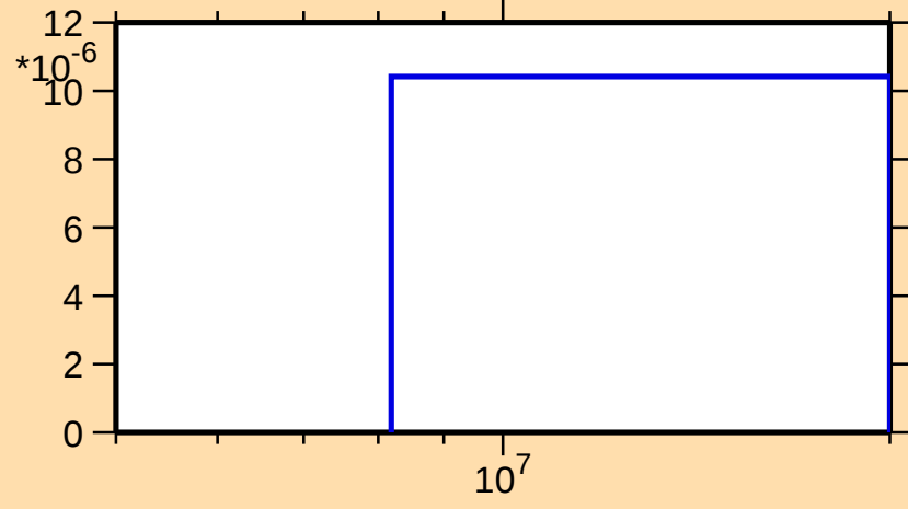
\sigma vs. E for ^{187}\text{Tl}(n,2np)
