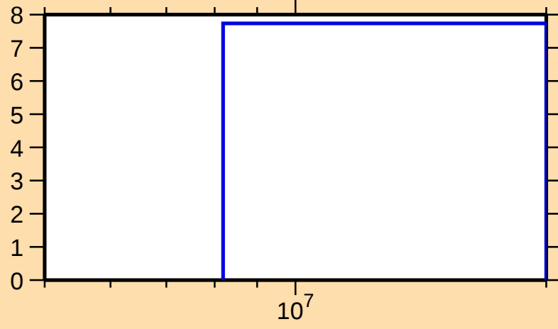
\Delta\sigma/\sigma vs. E for ^{187}\text{Tl}(n,\text{nonel.})
