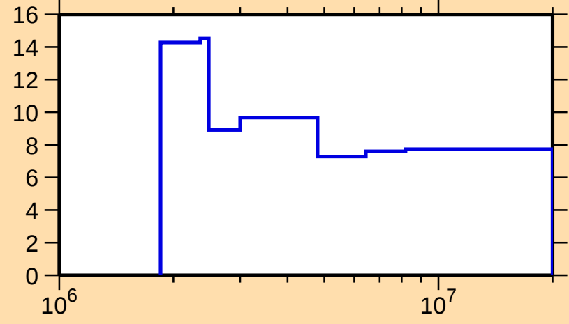
\Delta\sigma/\sigma vs. E for ^{187}\text{Tl}(n,n\text{nonel.})
