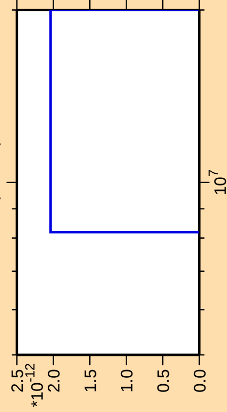
\Delta\sigma/\sigma vs. E for ^{187}\text{Tl}(\text{mt } 42)
