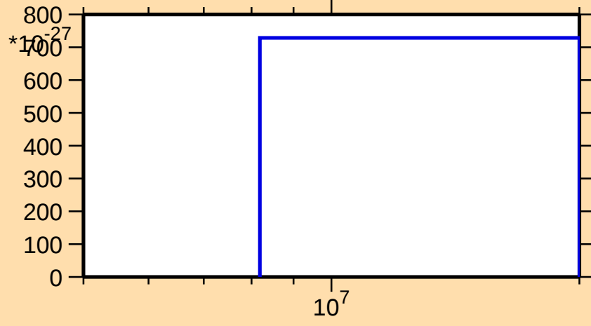
\sigma vs. E for ^{187}\text{Tl}(\text{mt } 42)
