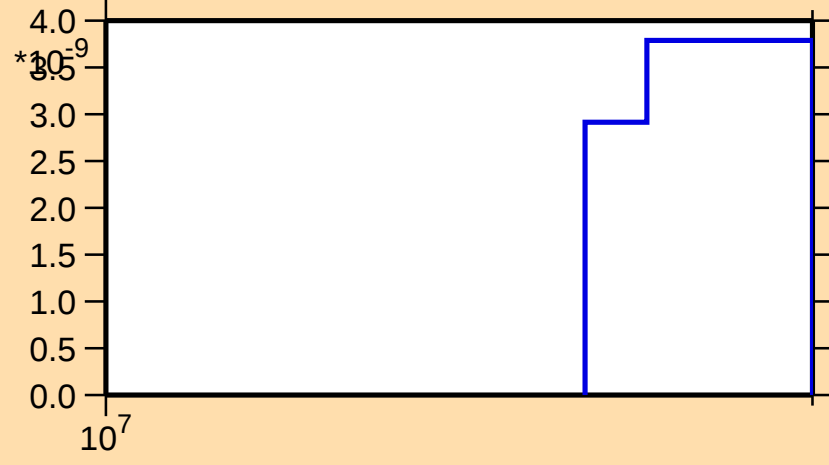
\sigma vs. E for ^{188}\text{Tl}(n,3n\alpha)
