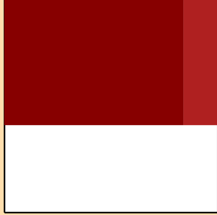
\Delta\sigma/\sigma vs. E for ^{188}\text{Tl}(n,\text{el.})
