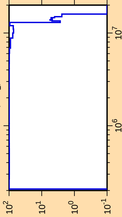
\Delta\sigma/\sigma vs. E for ^{188}\text{Tl}(n,n_1)
