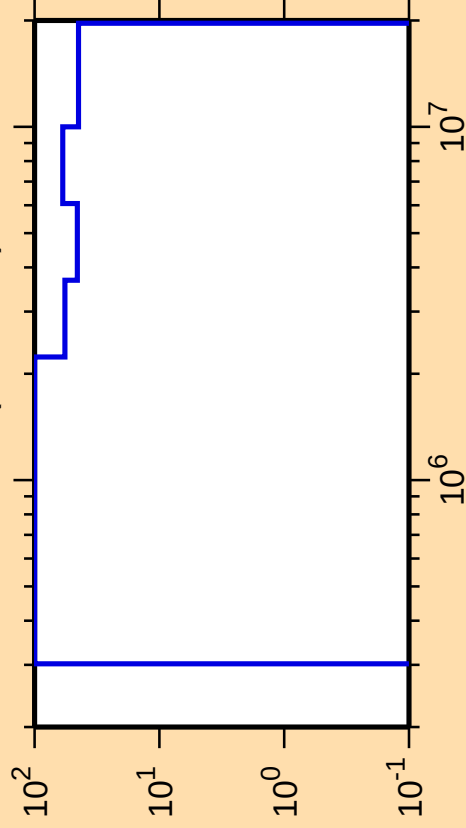
\Delta\sigma/\sigma vs. E for ^{188}\text{Tl}(n,n_{\text{cont}})
