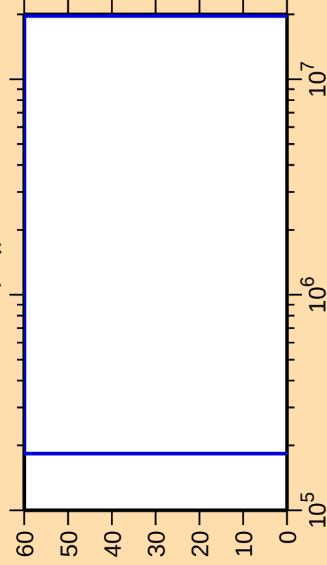
\Delta\sigma/\sigma vs. E for ^{188}\text{Tl}(n,\gamma)
