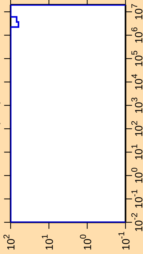
\Delta\sigma/\sigma vs. E for ^{188}\text{Tl}(n,\alpha)
