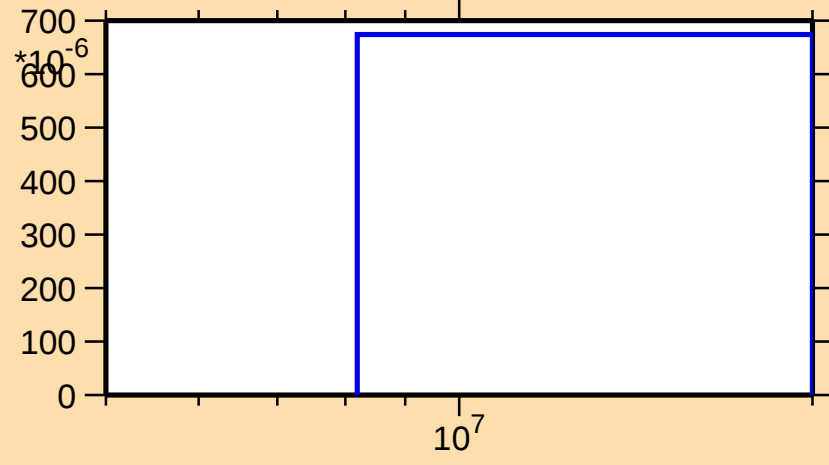
\sigma vs. E for ^{188}\text{Tl}(n,2np)
