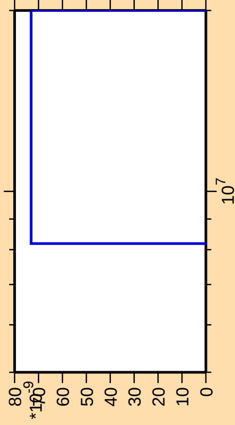
\Delta\sigma/\sigma vs. E for ^{188}\text{Tl}(\text{mt } 42)
