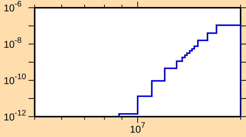
\sigma vs. E for ^{188}\text{Tl}(\text{mt117})
