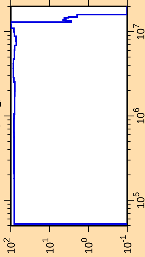
\Delta\sigma/\sigma vs. E for ^{188}\text{Tl}(n,n_2)
