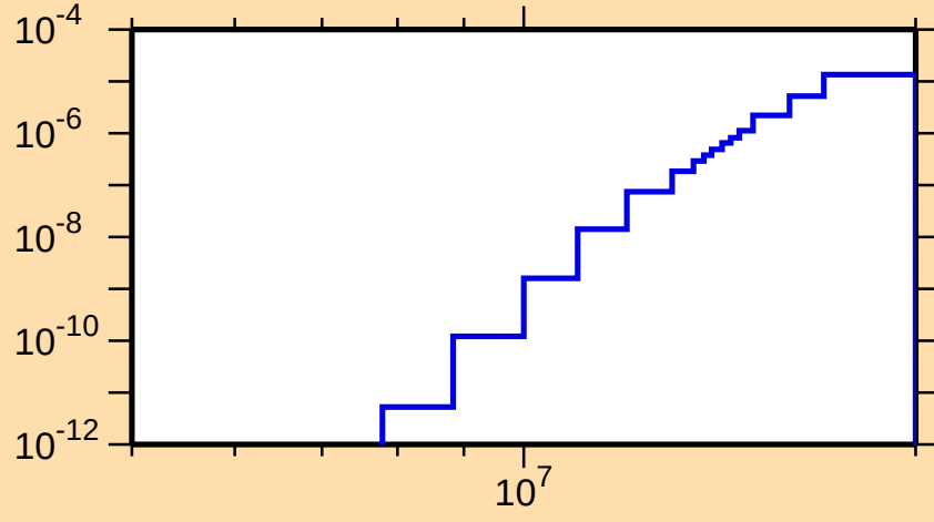
\sigma vs. E for ^{188}\text{Tl}(\text{mt } 45)
