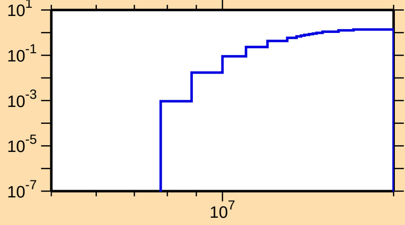
\sigma vs. E for ^{188}\text{Tl}(n,2n)
