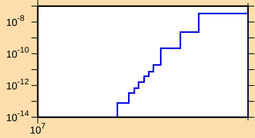
\sigma vs. E for ^{188}\text{Tl}(n,\text{pt})
