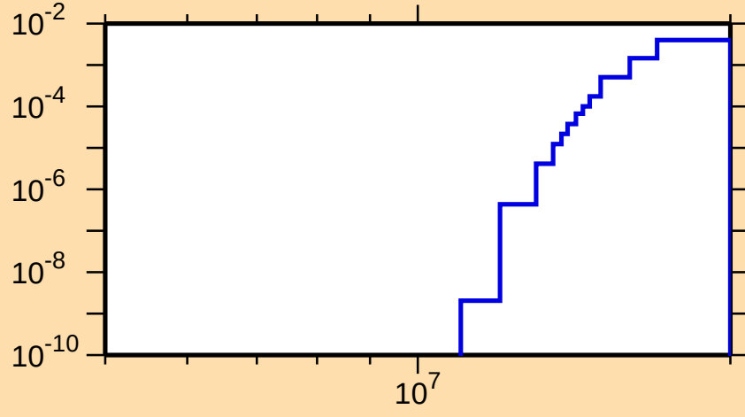
\sigma vs. E for ^{188}\text{Tl}(n,2np)
