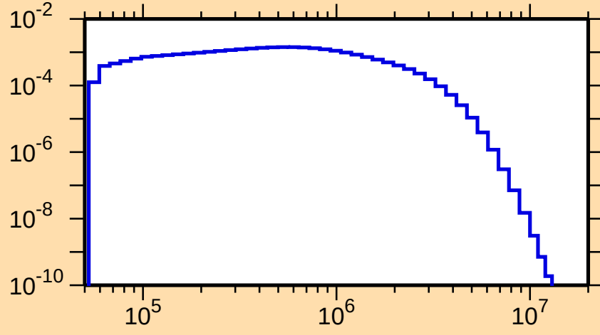
\sigma vs. E for ^{188}\text{Tl}(n,n_2)
