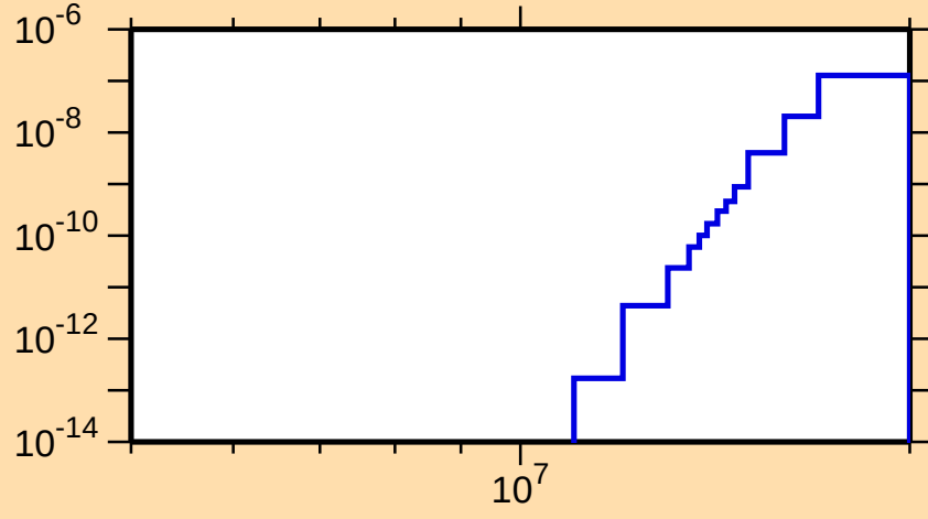
\sigma vs. E for ^{188}\text{Tl}(n,\text{pd})
