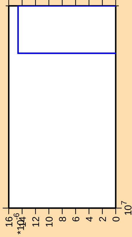
\Delta\sigma/\sigma vs. E for ^{188}\text{Tl} (mt 42)
