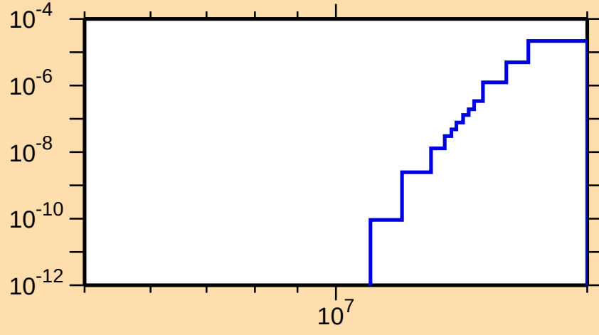
\sigma vs. E for ^{188}\text{Tl}(n,\text{nd})
