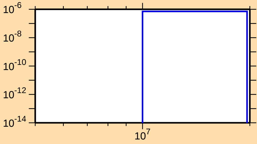
\sigma vs. E for ^{188}\text{Tl}(n,\text{nd})
