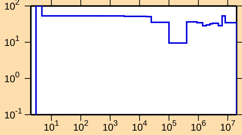
\Delta\sigma/\sigma vs. E for ^{188}\text{Tl}(n,\text{el.})
