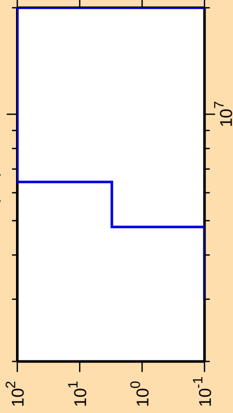
\Delta\sigma/\sigma vs. E for ^{188}\text{Tl}(n,t)
