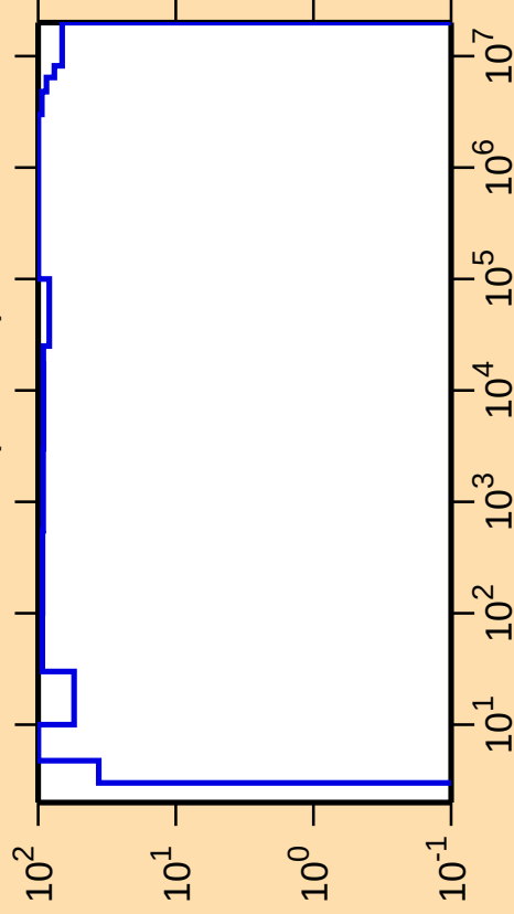
\Delta\sigma/\sigma vs. E for ^{188}\text{Tl}(n,\text{inel.})
