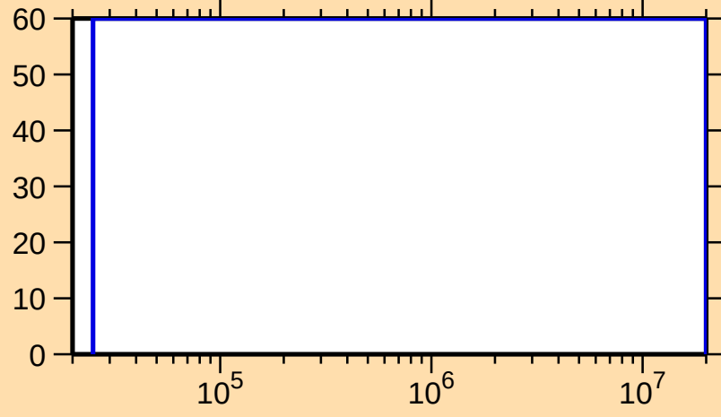
\Delta\sigma/\sigma vs. E for ^{188}\text{Tl}(n,n\text{cont.})
