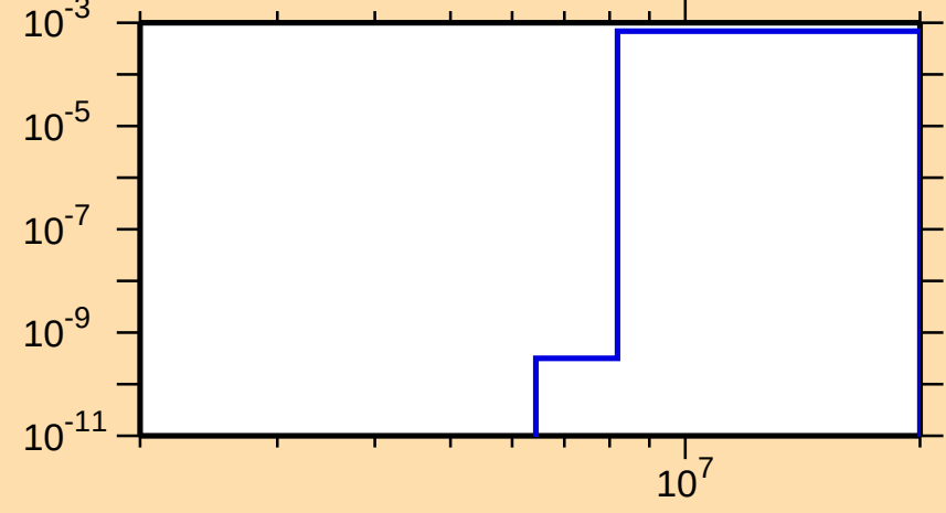
\sigma vs. E for ^{188}\text{Tl}(n,t)
