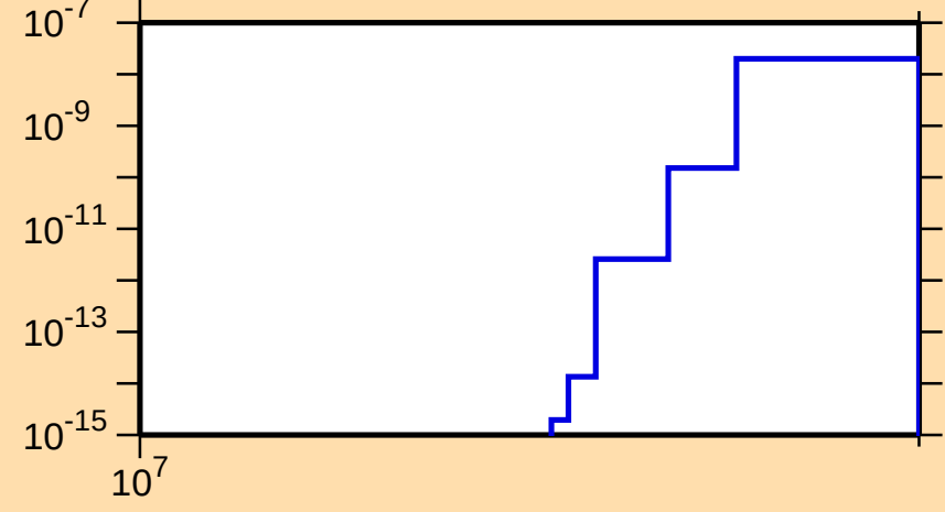
\sigma vs. E for ^{189}\text{Tl}(n,\text{nt})
