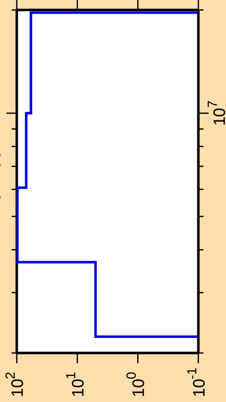
\Delta\sigma/\sigma vs. E for ^{189}\text{Tl}(n,np)
