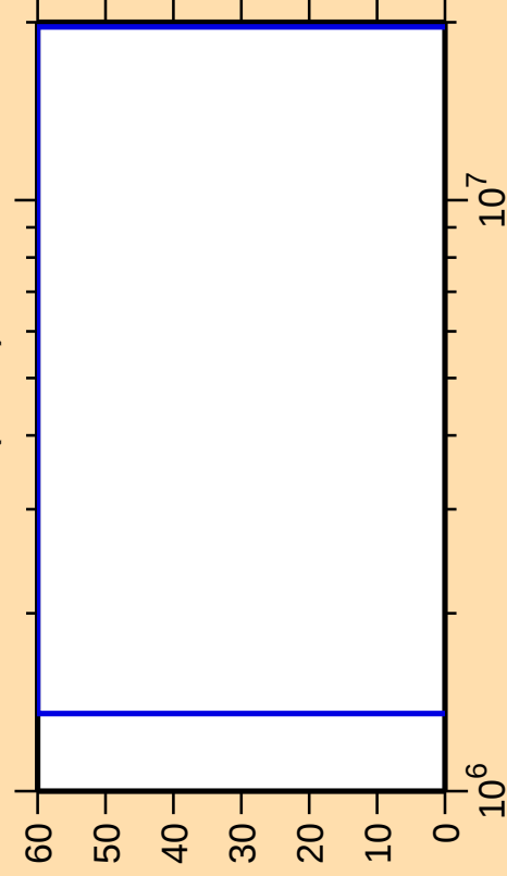
\Delta\sigma/\sigma vs. E for ^{189}\text{Tl}(n,n\alpha)
