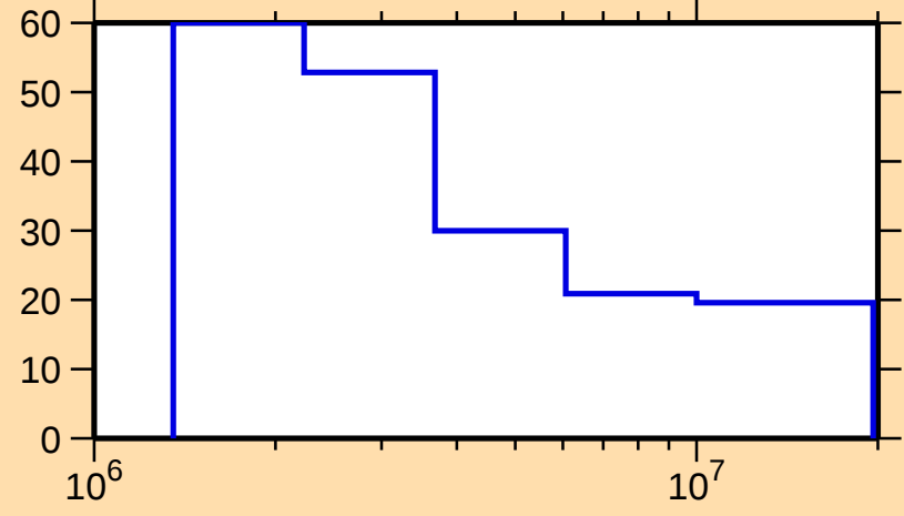
\Delta\sigma/\sigma vs. E for ^{189}\text{Tl}(n,ncont.)
