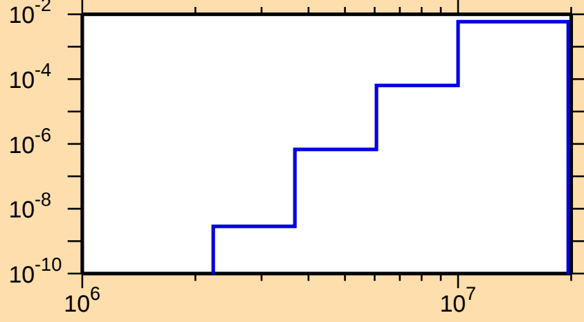
\sigma vs. E for ^{189}\text{Tl}(n,n\alpha)
