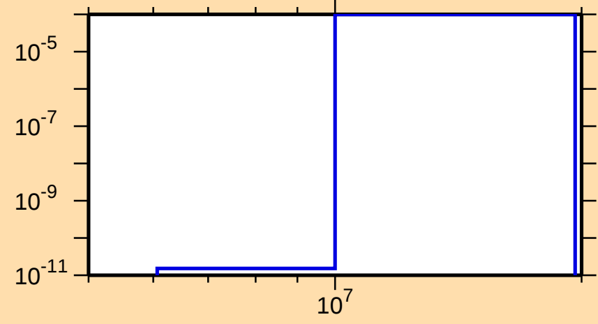
\sigma vs. E for ^{189}\text{Tl}(n,t)
