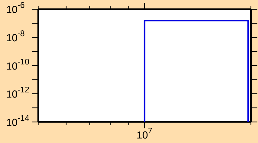
\sigma vs. E for ^{189}\text{Tl}(n,2n\alpha)
