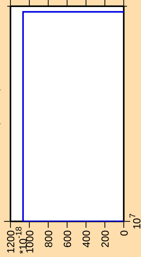
\Delta\sigma/\sigma vs. E for ^{189}\text{Tl}(\text{mt } 42)
