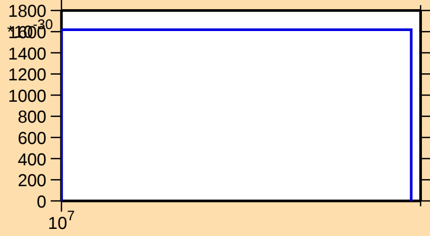
\sigma vs. E for ^{189}\text{Tl}(\text{mt } 42)
