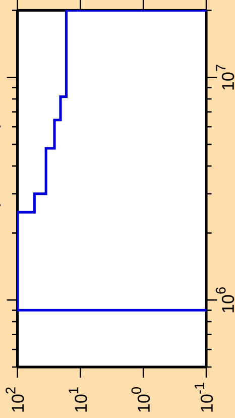
\Delta\sigma/\sigma vs. E for ^{189}\text{Tl}(n,n_{\text{cont}})
