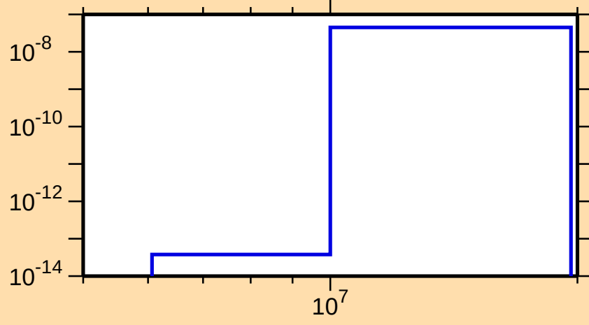
\sigma vs. E for ^{190}\text{Tl}(\text{mt } 45)
