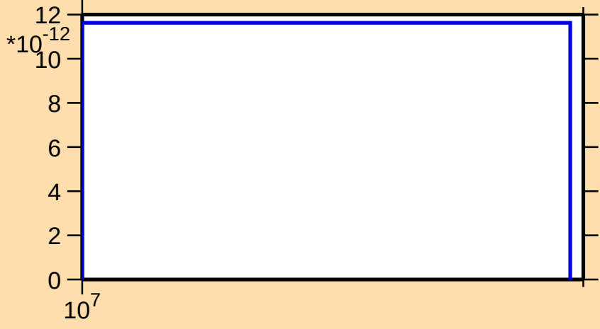
\sigma vs. E for ^{190}\text{Tl}(n,\text{pt})
