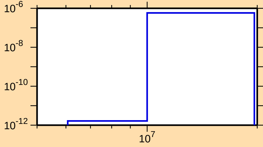
\sigma vs. E for ^{190}\text{Tl}(n,\text{He}3)
