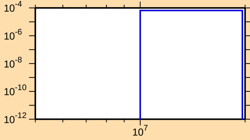
\sigma vs. E for ^{190}\text{Tl}(n,2np)
