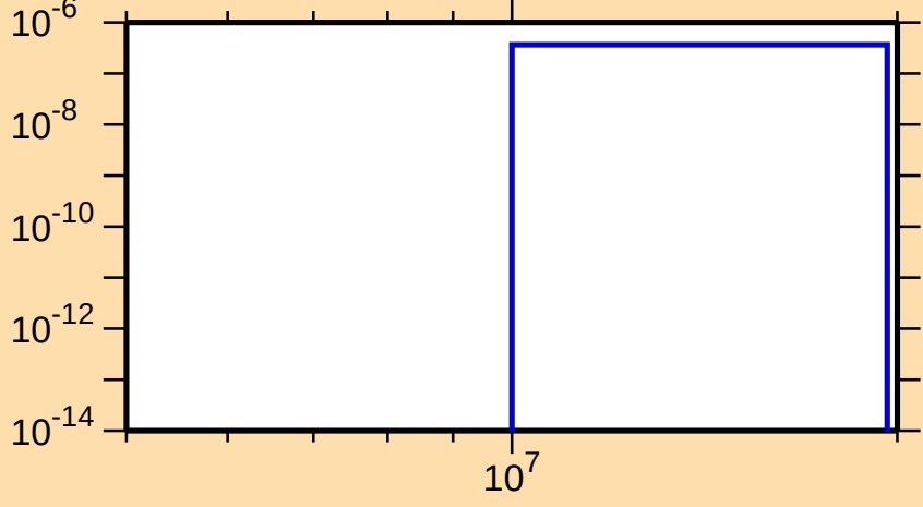
\sigma vs. E for ^{190}\text{Tl}(n,\text{nd})
