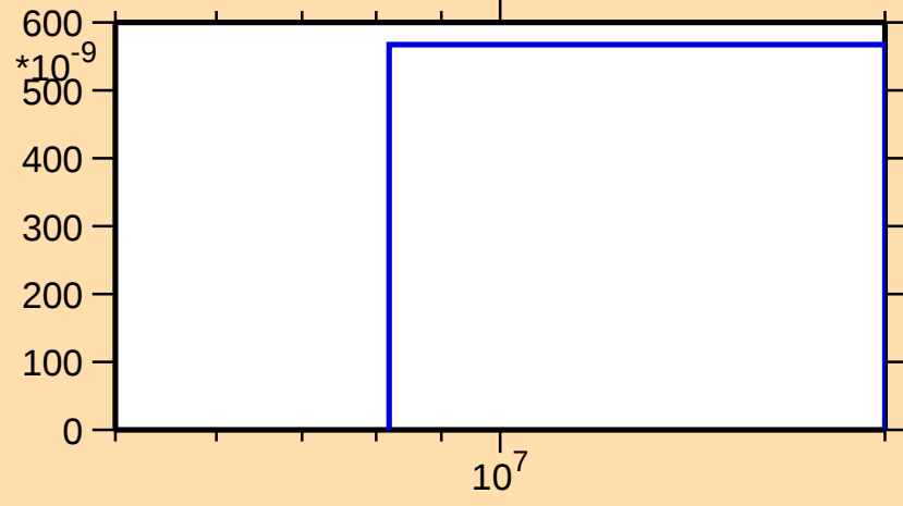
\sigma vs. E for ^{190}\text{Tl}(n,3n)
