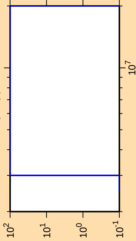
\Delta\sigma/\sigma vs. E for ^{190}\text{Tl}(n,np)
