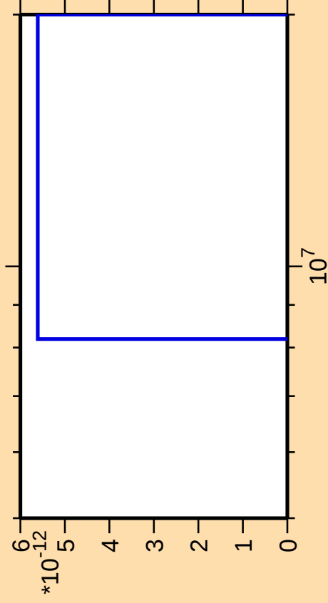
\Delta\sigma/\sigma vs. E for ^{190}\text{Tl}(\text{mt } 42)
