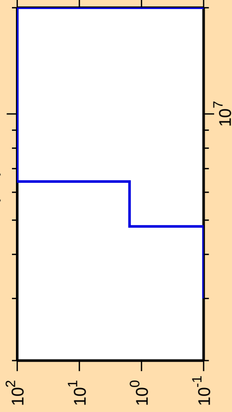
\Delta\sigma/\sigma vs. E for ^{190}\text{Tl}(n,t)
