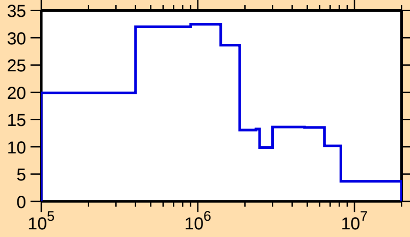
\Delta\sigma/\sigma vs. E for ^{190}\text{Tl}(n,\text{tot.})
