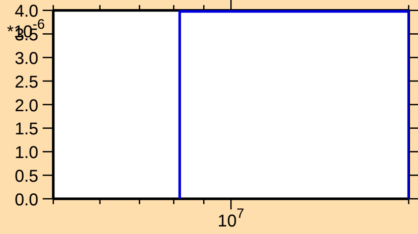
\sigma vs. E for ^{190}\text{Tl}(n,2n\alpha)
