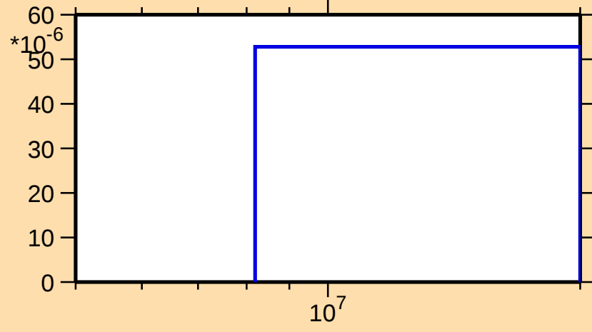
\sigma vs. E for ^{190}\text{Tl}(n,2np)
