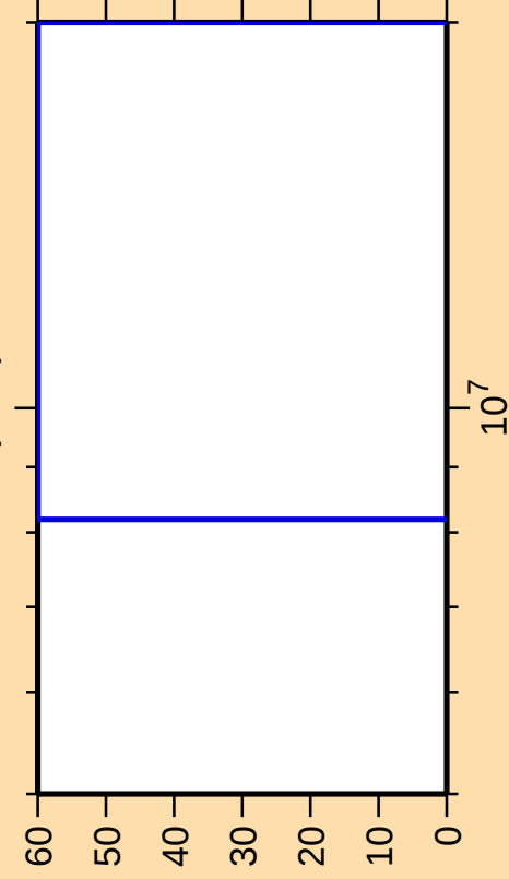
\Delta\sigma/\sigma vs. E for ^{190}\text{Tl}(n,\text{nt})
