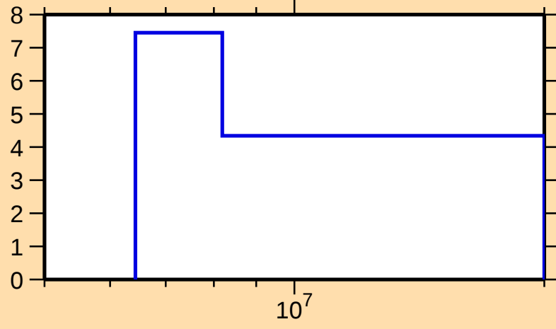
\Delta\sigma/\sigma vs. E for ^{190}\text{Tl}(n,\text{nonel.})
