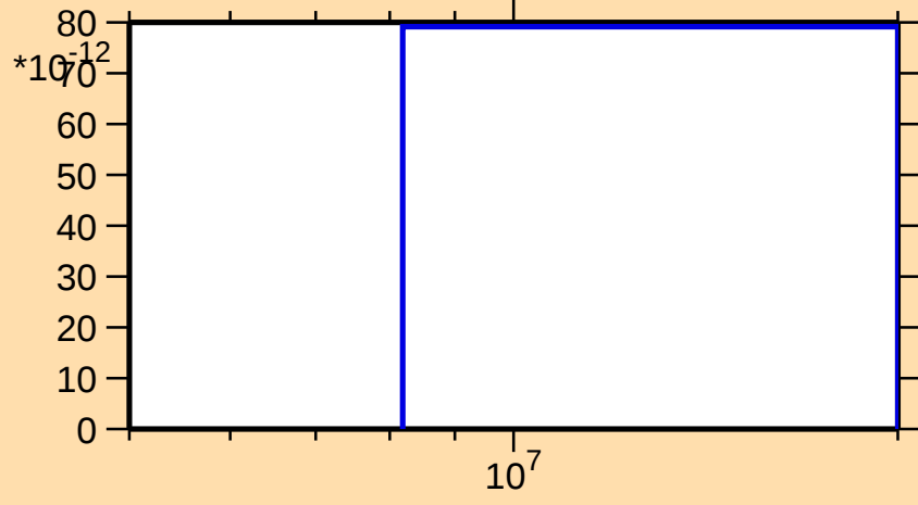
\sigma vs. E for ^{190}\text{Tl}(n,\text{nt})
