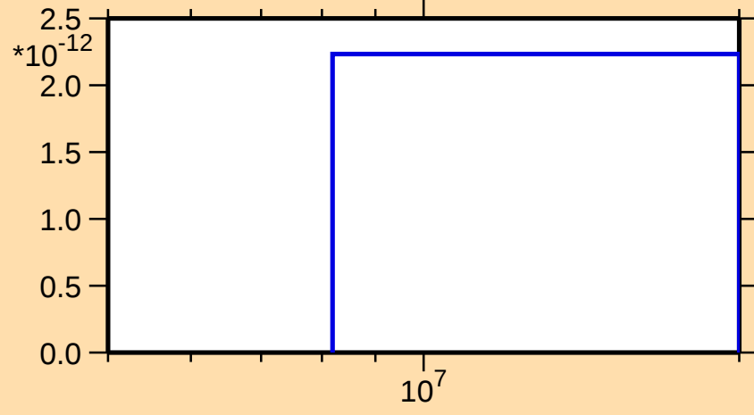
\sigma vs. E for ^{190}\text{Tl}(\text{mt 34})
