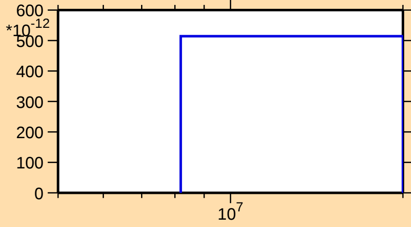
\sigma vs. E for ^{190}\text{Tl}(\text{mt117})
