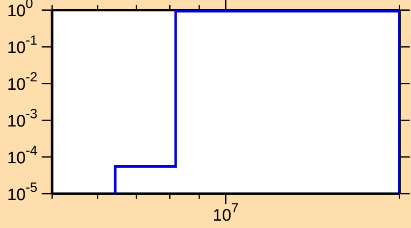
\sigma vs. E for ^{190}\text{Tl}(n,2n)
