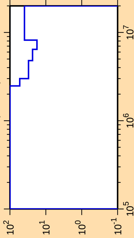
\Delta\sigma/\sigma vs. E for ^{190}\text{Tl}(n,\text{inel.})
