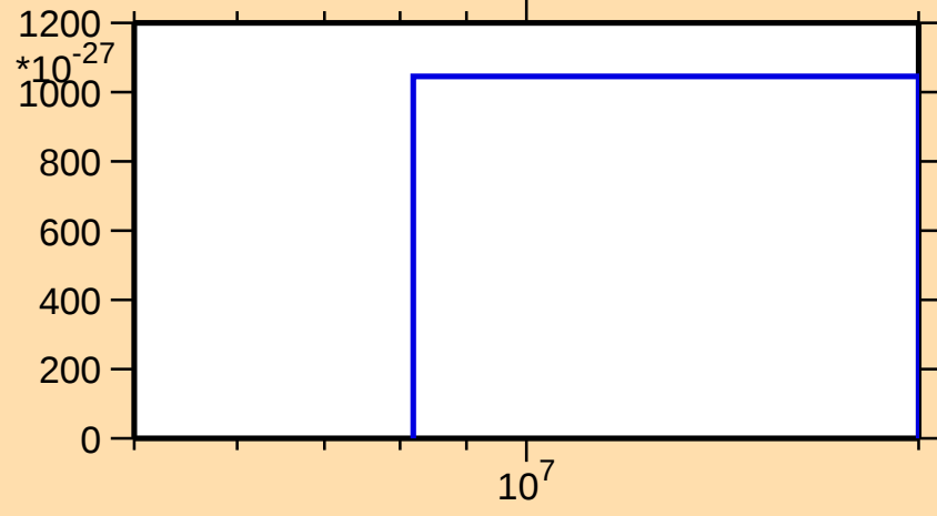
\sigma vs. E for ^{190}\text{Tl}(\text{mt } 42)
