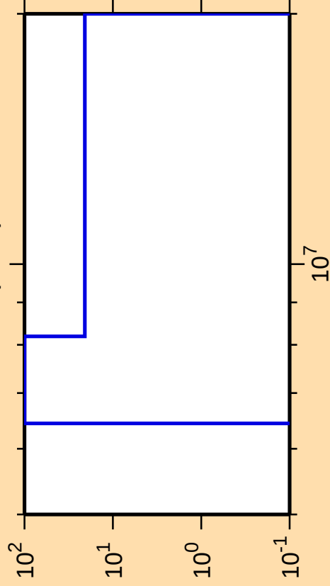
\Delta\sigma/\sigma vs. E for ^{190}\text{Tl}(n,2n)
