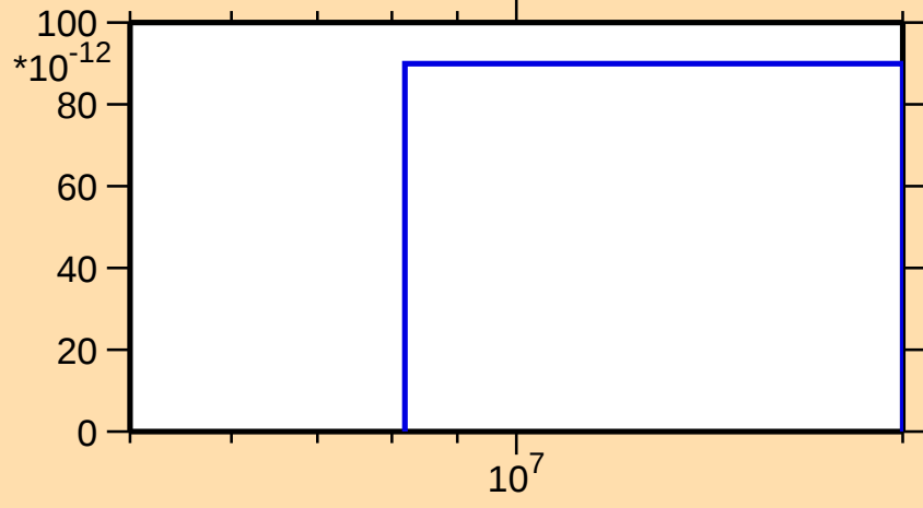
\sigma vs. E for ^{190}\text{Tl}(n,\text{pd})
