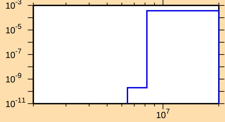
\sigma vs. E for ^{190}\text{Tl}(n,t)
