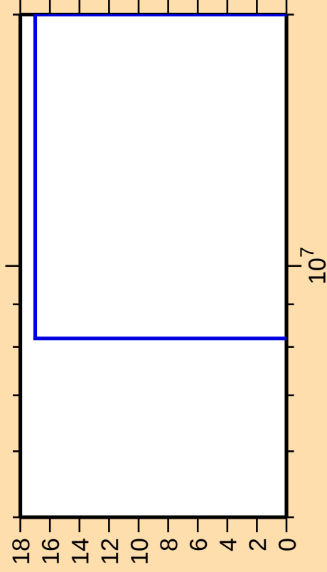
\Delta\sigma/\sigma vs. E for ^{190}\text{Tl}(\text{mt 34})
