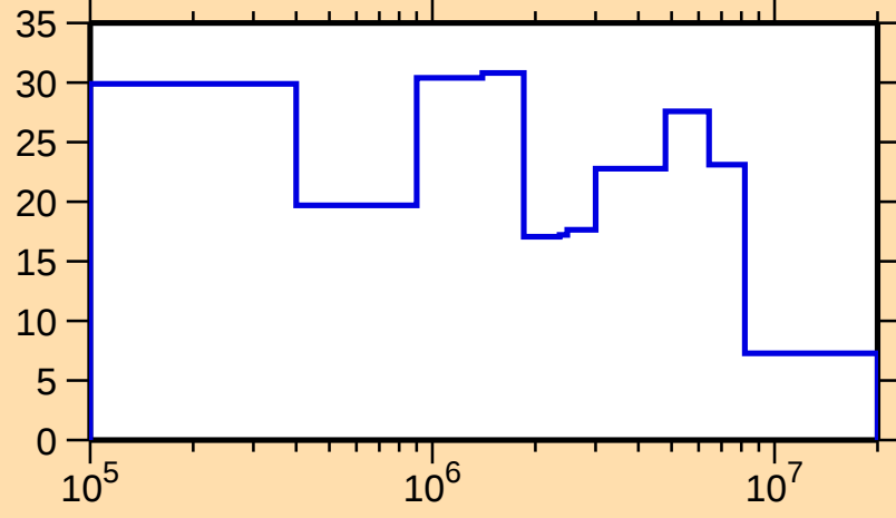
\Delta\sigma/\sigma vs. E for ^{190}\text{Tl}(n,\text{el.})
