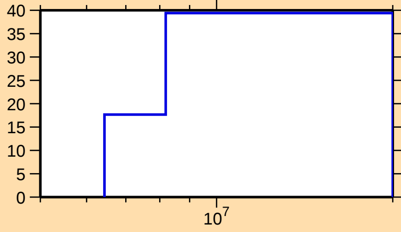
\Delta\sigma/\sigma vs. E for ^{190}\text{Tl}(n,\text{inel.})
