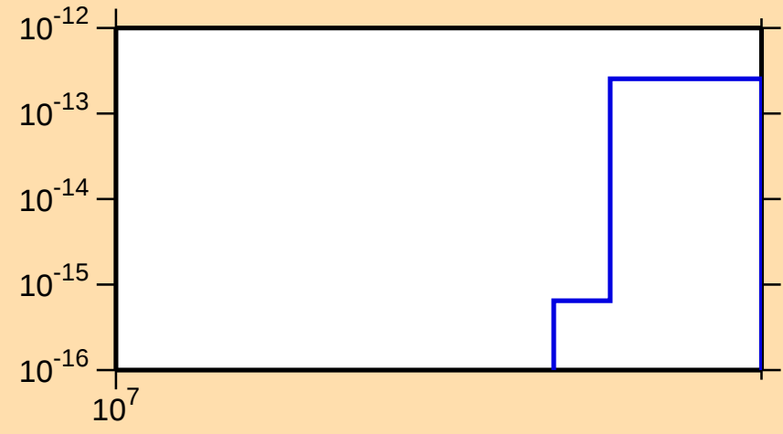
\sigma vs. E for ^{191}\text{Tl} (mt 34)
