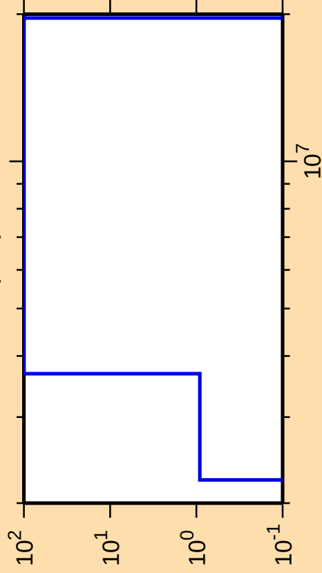
\Delta\sigma/\sigma vs. E for ^{191}\text{Tl}(n,d)
