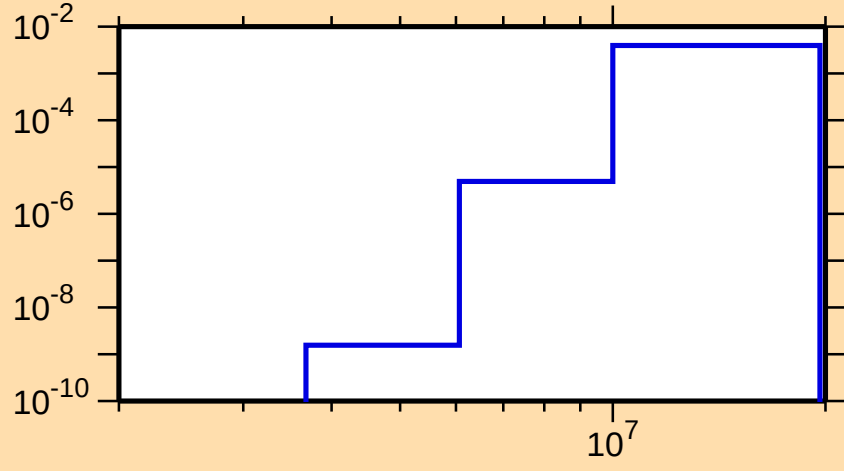
\sigma vs. E for ^{191}\text{Tl}(n,d)
