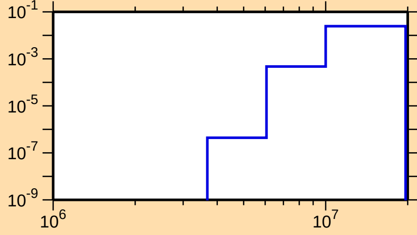
\sigma vs. E for ^{191}\text{Tl}(n,np)
