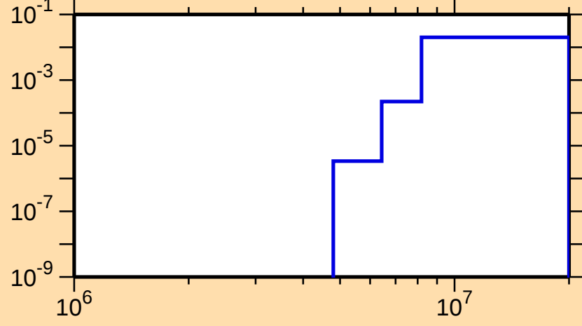
\sigma vs. E for ^{191}\text{Tl}(n,np)
