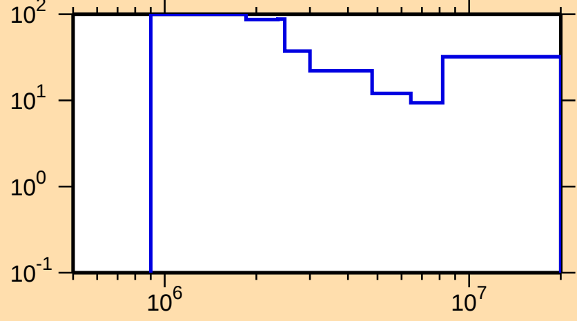
\Delta\sigma/\sigma vs. E for ^{191}\text{Tl}(n,n\text{cont.})
