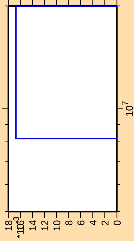
\Delta\sigma/\sigma vs. E for ^{191}\text{Tl} (mt 34)
