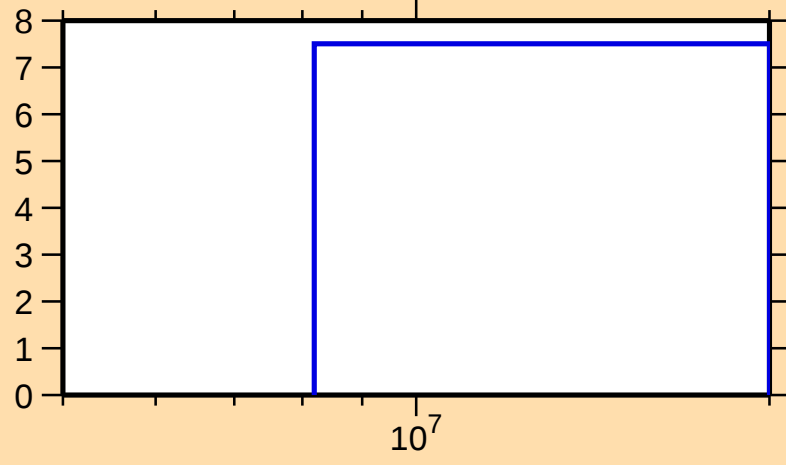
\Delta\sigma/\sigma vs. E for ^{191}\text{Tl}(n,\text{el.})
