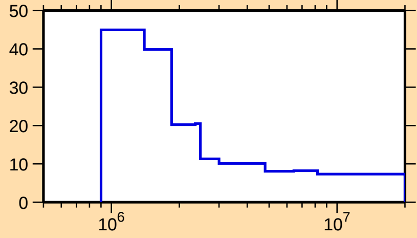
\Delta\sigma/\sigma vs. E for ^{191}\text{Tl}(n,n\text{nonel.})
