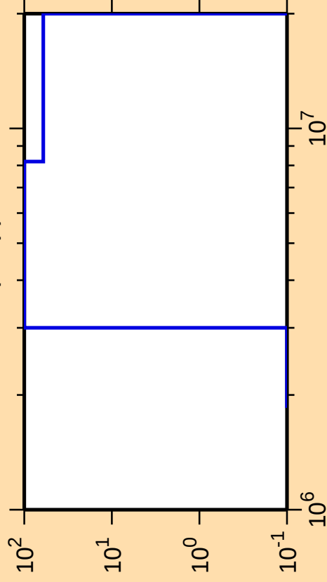
\Delta\sigma/\sigma vs. E for ^{191}\text{Tl}(n,np)
